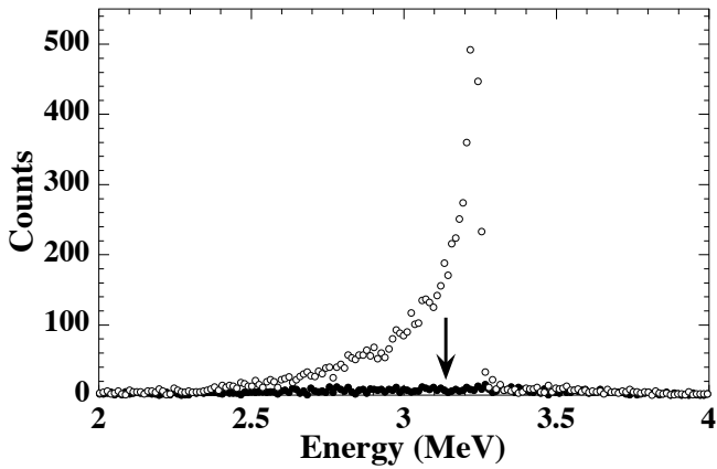
FIG. 2: \alpha spectra from ^{18}\text{O}(p,\alpha)^{15}\text{N} : E_p = 629 keV. (o) porous Si layer after thermal oxidation in ^{18}\text{O}_2 ( A_o ). (●) part of the layer protected by Al cap ( A_c ). The arrow indicates the energy of the expected \alpha peak from A_c .
