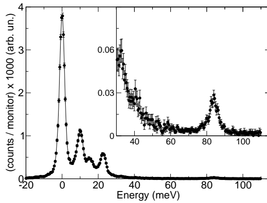
FIG. 1: Inelastic x-ray scattering example spectrum of \text{La}_{1.86}\text{Ba}_{0.14}\text{CuO}_{4+\delta} , at \mathbf{Q} = (3.11, 0.04, 0) . At zero energy one observes the elastic line, while at positive energy, several phonon modes are observed corresponding to Stokes processes. In the inset we zoom on to the high energy optical Cu-O bond stretching mode. Anti-Stokes modes are not visible because of the unfavorable detailed balance at low temperature.
