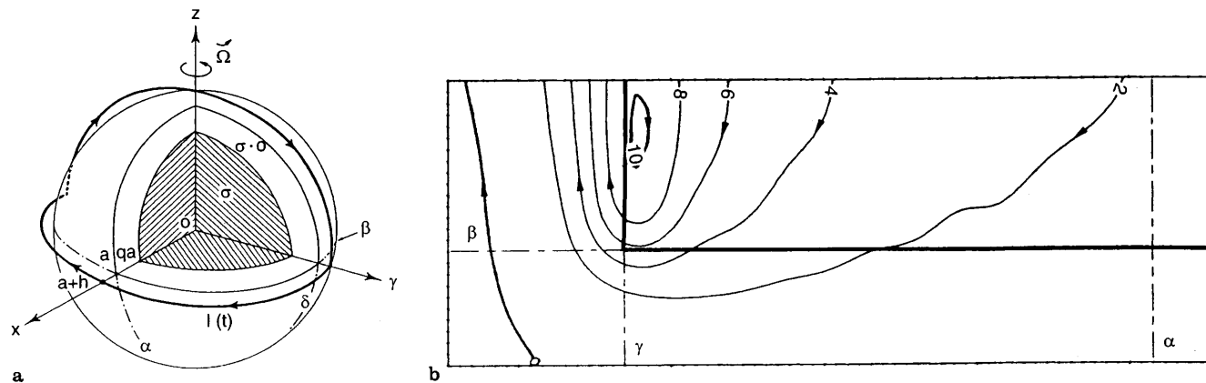
Fig. 6. A External current model and Earth conductivity Ducruix et al. 's (1977) model in the spherical case. Coordinate system Oxyz ( r, q, l ) is fixed with respect to the Earth. Current circuit (shown as a thick line, comprises a half equatorial circle and two half meridians on the sphere with radius R = a + h , where a is the Earth radius and h the ionospheric altitude. The uniform conductive core has radius qa and conductivity s . The current circuit rotates with velocity \mathbf{W} = (2p/T_0) \mathbf{z} , with T_0 = 24 h. Parameters used by Ducruix et al. (1977) are
