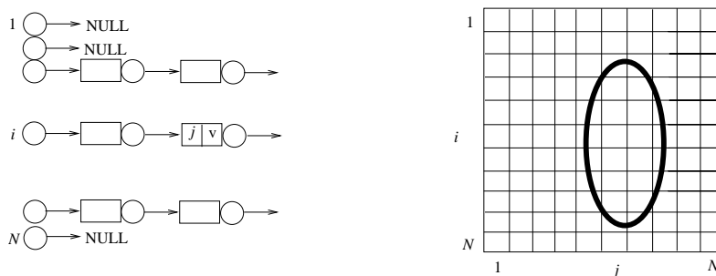
Figure 3: a sparse semi-dynamic linked structure storing the nodes
