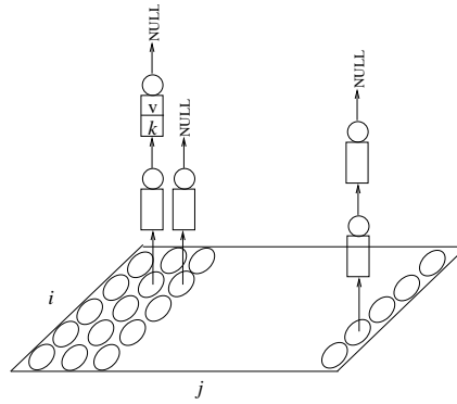
Figure 4: SSD structure in three dimensions
