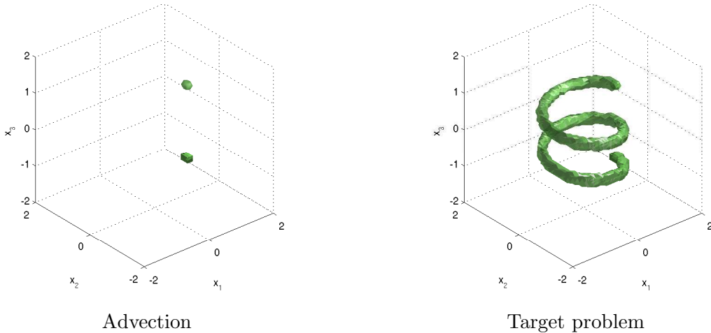
Figure 9: (Example 4) advection problem (left), target problem (right). T = 2 , N = 50 .
