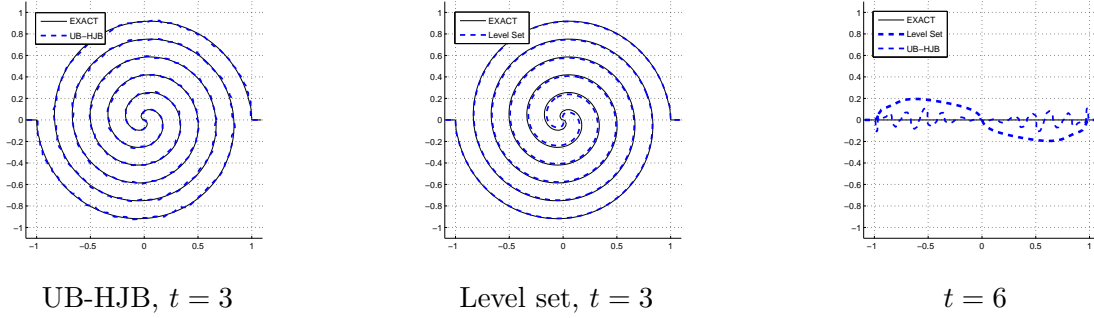
Figure 7: (Example 3) UB-HJB and level set methods at times t = 3 (after three turns) and t = 6 (return to initial data), CFL=0.9, with N = 100 .
