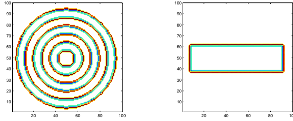
Figure 5: Fronts for example 1 (left) and example 2 (right).
