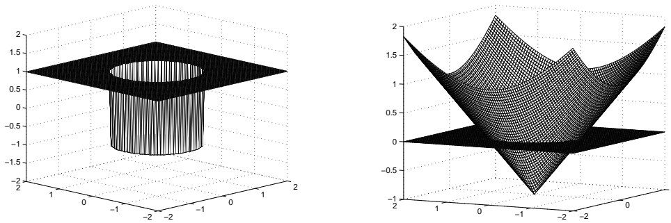
Figure 1: Discontinuous approach (left) vs. level set approach (right)
