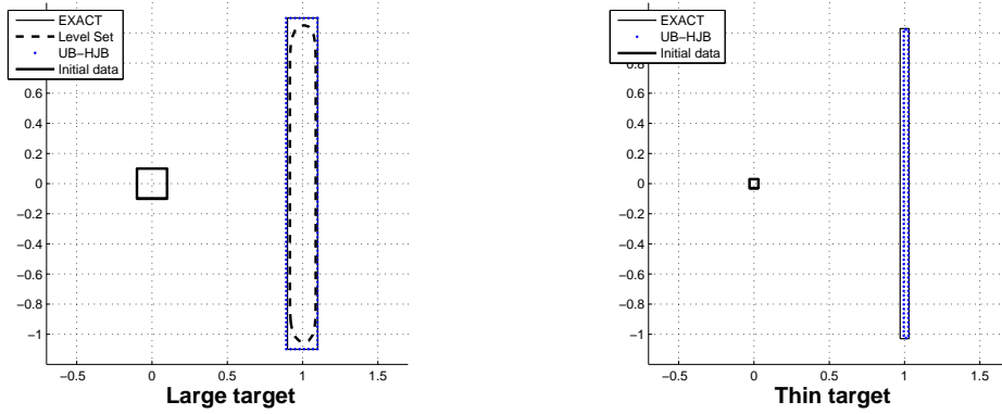
Figure 6: (Example 2) Rendez vous problem with N = 101 .
