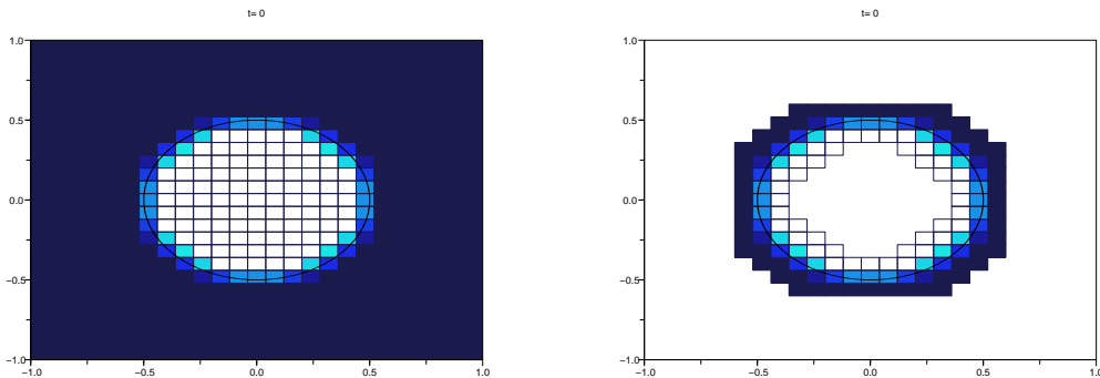
Figure 2: Full (left) and sparse (right) matrix coding.
