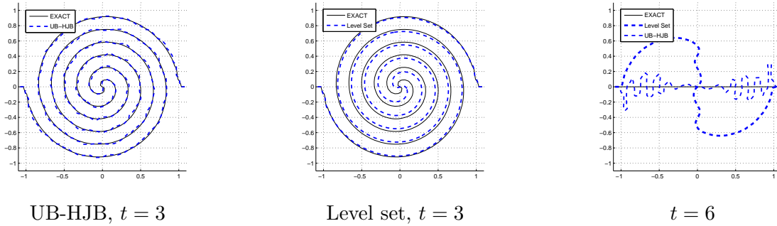
Figure 8: (Example 3) Same computation as in Fig. 7, with N = 50 .
