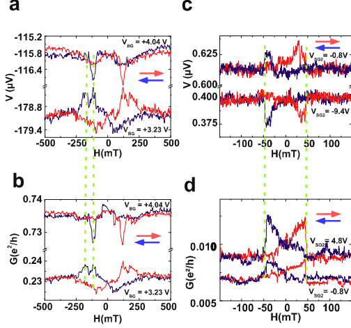
FIG. 5: a. Non-local voltage V_{34} for sample II as a function of the external magnetic field H for V_{SG1} = 0.00V , V_{SG2} = 0.00V and V_{BG} = 4.04V or V_{BG} = 3.23V . b. Similar plot for G of sample II. c. Non-local voltage V_{34} for sample III as a function of H for V_{SG1} = -5.00V , V_{BG} = -5.455V and V_{SG2} = -9.4V or V_{SG2} = -0.8V . d. Similar plot for G of sample III for V_{SG1} = -5.00V , V_{BG} = -5.455V and V_{SG2} = 4.8V or V_{SG2} = -0.8V .
