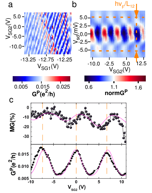
FIG. 6: a. Colorscale plot of G^P as a function of V_{SG1} and V_{SG2} for sample III. b. Colorscale plot of the normalized G of sample III as a function of V_{sd} and V_{SG2} . c. Simultaneous variations of MG and G^P as a function of V_{SG2} for sample III.
