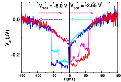
FIG. 4: Non-local voltage V_{34} for sample I as a function of the external magnetic field H for V_{SG2} = -6.0V and -2.65V . The curves for V_{SG2} = -2.65V has been shifted up to make them coincide with those for V_{SG2} = -6.0V at zero field.
