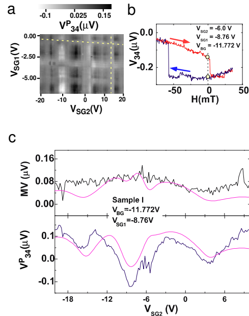
FIG. 3: a. Greyscale plot showing the "tartan" pattern of the non local voltage V_{34}^P of sample I in the P configuration. b. "Minor hysteresis loop" for the non-local voltage V_{34} of sample I for V_{SG1} = -8.76V , V_{SG2} = -6.00V and V_{BG} = -11.772V . c. V_{34}^P and MV as a function of V_{SG2} . In purple, the prediction from the multi-terminal scattering theory of ref. 27 with the parameters described in the appendix.
