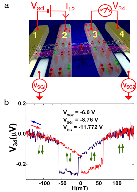
FIG. 1: a. Schematics diagram of the devices studied in the article. b. Non-local voltage V_{34} for sample I as a function of the external magnetic field H for side gate voltages V_{SG1} = -8.76V , V_{SG2} = -6.00V and a back gate voltage V_{BG} = -11.772V .
