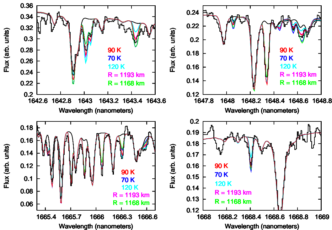
Fig. 3. Model fitting of the August 1, 2008 Pluto spectrum (histograms) zoomed on four spectral regions. The black curve is a model with no methane on Pluto. The 90 K, 70 K, and 120 K curves indicate isothermal, single-layer, fits, including 0.75 cm-am, 1.3 cm-am and 0.45 cm-am of \text{CH}_4 , respectively. The rotational distribution of lines indicates that a 90 K temperature provides the best fit. The “R= 1193 km” model (pink, fit almost indistinguishable to the 90 K model) corresponds to a 6 K/km stratospheric temperature gradient, a 1193 km radius (7.5 \mu\text{bar} surface pressure) and a 0.62 % methane mixing ratio. The “R=1168 km” model includes a 6 K/km stratospheric temperature gradient, joining with a wet tropospheric lapse rate of -0.1 K/km below 1188 km (tropopause) and extending down to a 1168 km surface radius (29 \mu\text{bar} ). This 20 km-deep troposphere model, optimized here with \text{CH}_4 = 0.36\% , is inconsistent with the methane spectrum; for this thermal profile, the minimum radius is 1172 km (see Fig. 4) . The wavelength scale is in the observer frame. These spectral regions are those showing maximum sensitivity to the methane temperature (or equivalently depth of the troposphere), as they include low J-level and high J-level lines, but for quantitative analysis, a least-square fit on all lines was performed.
