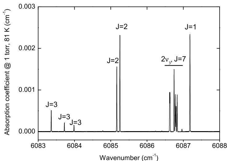
Fig. 2. Laboratory spectrum of methane at 81 K in the 6083-6088 \text{cm}^{-1} range, demonstrating the existence of strong, low J-level, lines in addition to the R-branch manifolds of the 2\nu_3 band. The J-level for these lines is determined by comparison of their intensity at 81 K and at room temperature (see Gao et al. 2009). The J=2 doublet near 6085.2 \text{cm}^{-1} is marginally detected in the Pluto spectrum (1643.4 nm, see Fig. 3).
