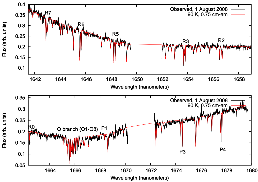
Fig. 1. Black: Pluto spectrum observed with VLT/CRIRES. Red: Best-fit isothermal model (90 K, 0.75 cm-am \text{CH}_4 ), including telluric and solar lines. The general continuum shape is due to absorption in the 2\nu_2 + \nu_3 and 2\nu_3 bands of solid methane (see Douté et al. 1999)
