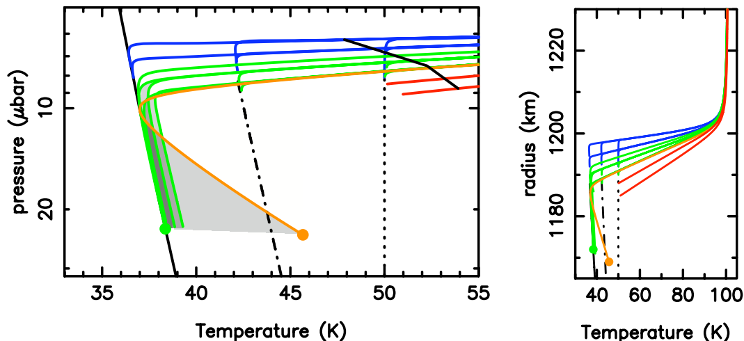
Fig. 4. Range of possible thermal profiles (pressure-temperature (left) and radius-temperature (right)) in Pluto's atmosphere. From bottom to top, they have stratospheric thermal gradients of 3 and 4 K/km (red profiles), 5 K/km (one orange and one green), 6 K/km (two green), 7 K/km (green), and 9 and 15 K/km (blue). All profiles are continuous in first and second order temperature derivatives. Most of these profiles have no or very limited tropospheres (less than 5 km in depth), in order to match the residual flux observed during stellar occultations and avoid the formation of strong caustics (see Fig. 5). Only profiles in green and orange, with moderate stratospheric temperature gradients (5-7 K/km) and a cold tropopause ( < 38 K) can have significant tropospheres. The lapse rate in such tropospheres ranges from -0.1 K/km, corresponding to the N_2 wet adiabat (green profiles) to -0.6 K/km ( N_2 dry adiabat, orange profile). The CRIRES spectra indicate that these wet and dry profiles cannot extend deeper than p \sim 24 \mu\text{bar} (1172 and 1169 km, respectively). In the left panel, the solid line on the top right is the locus of minimum atmospheric pressure implied by the observation of a central flash, and the solid line on the left is the vapour pressure equilibrium of N_2 . The dashed-dotted line is the vapour pressure equilibrium of CH_4 for a 0.5 % mixing ratio. The dotted line at 50 K illustrates the maximum possible near-surface gas temperature. The shaded areas represent the range of possible tropospheres. If Pluto has a troposphere, methane must be supersaturated over most of it.
