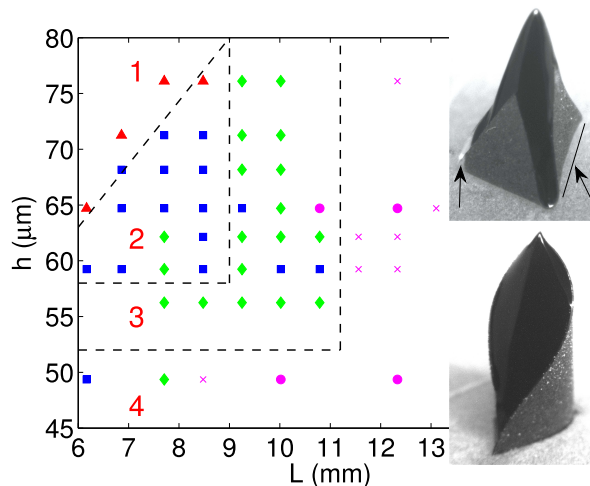
FIG. 5. (Color online) Main: Phase diagram of the origami configuration before instability as a function of membrane length, L , and thickness, h : no origami (▲), usual origami (■), origami with dewetting only (◼), with ridge curvature only (●), with ridge curvature and dewetting (×). Top inset: ferrofluid dewetting (see left arrow) and ridge curvature (see right arrow) before instability. Bottom inset: “Anomalous” final state after the instability when adhesion is involved.
