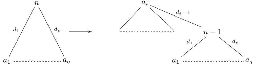
Figure 1: Rewriting rule on agents
