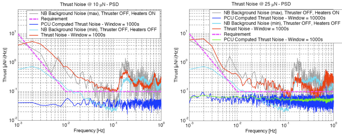
Figure 4. Thruster noise measured on the nano-balance facility for different thrust levels. The red line represents the measured thrust noise, while the grey line represents the facility noise during the test conditions. As can be seen the thrust noise measurement is limited by the facility background noise. The LPF requirement is shown in magenta. The blue data represents the calculated thrust noise as measured by the PCU from the current and voltage applied.
