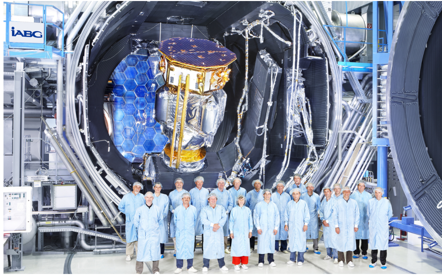
Figure 5. The LISA Pathfinder launch composite being in the vacuum chamber in preparation for the Transfer Orbit Thermal Balance test. The test was performed at the IABG, Germany.
