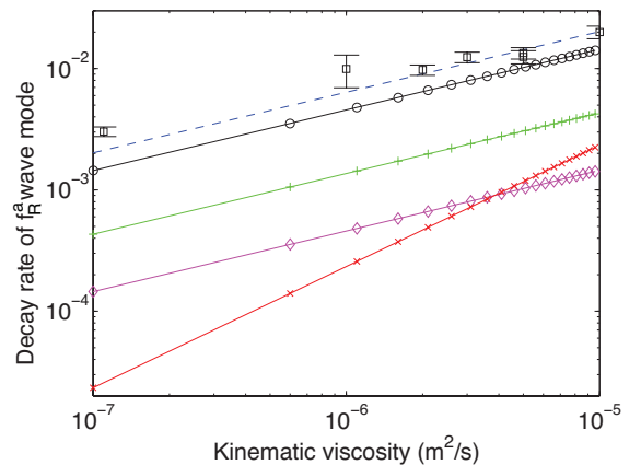
FIG. 7. (Color online) Decay rate, 1/(\tau 2\pi f_R^a) , of the wave mode at f_R^a = 3.2 Hz as a function of viscosity \nu for various fluids ( \square ). Theoretical decay rate by viscous dissipation: ( \circ ) surface boundary layer, \delta_S from Eq. (2), ( + ) bottom surface boundary layer, \delta_B from Eq. (3), ( \diamond ) wall surface layer, \delta_W from Eq. (4), and ( \times ) viscous surface \delta_\nu from Eq. (1). Dashed line is the total theoretical dissipation \delta_T = \delta_S + \delta_B + \delta_W .
