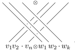
Figure 6: Pre-braiding extended to T(V)
