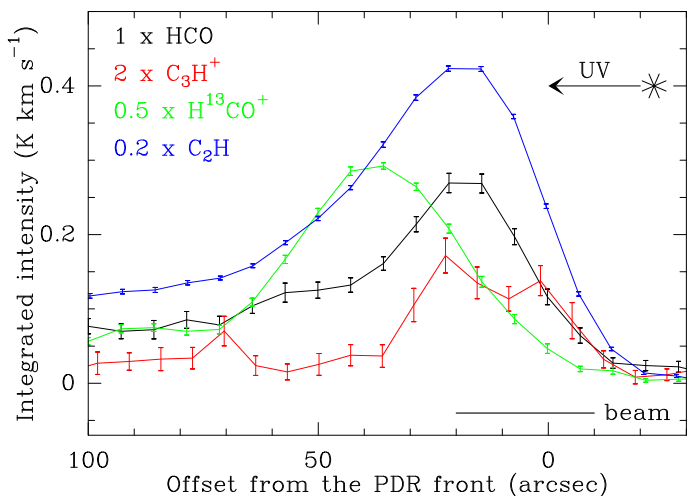
Fig. 3. Integrated intensity profiles across the PDR photo-dissociation front of the l\text{-C}_3\text{H}^+ , \text{HCO} , \text{H}^{13}\text{CO}^+ , and \text{C}_2\text{H} species (IRAM-30m). The cut would appear horizontal at \delta y = 0'' on Fig. 2. The observed lines are summarized in Table 2.
