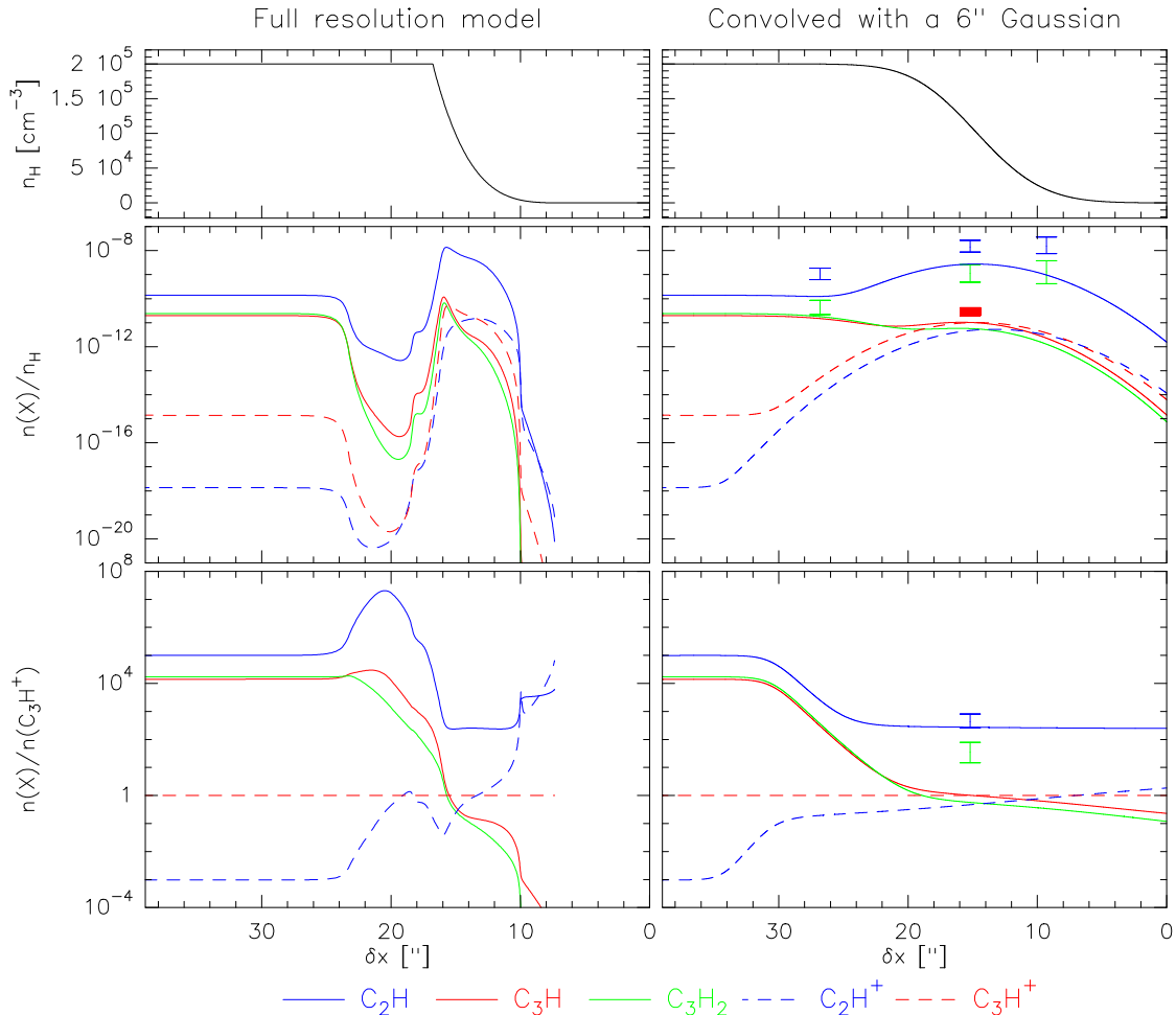
Fig. 5. Photochemical model of the Horsehead PDR displayed at the full resolution of the model ( left column ) and convolved with a Gaussian of 6''-FWHM ( right column ). Top: Horsehead density profile n_{\text{H}} = n(\text{H}) + 2n(\text{H}_2) . Middle: Predicted abundance of selected small hydrocarbons molecules and cations. Bottom: Abundances of the same hydrocarbons relative to the abundance of C 3 H + . The illuminating star is positioned at the right of the plots. The symbols present the measured range of possible abundances for C 2 H (blue vertical segment), C 3 H 2 (green vertical segment), and C 3 H + (red filled rectangle), inferred at a typical resolution of 6''. The legend at the bottom of the figure presents the line coding for the curves: C 2 H in plain blue, C 2 H + in dashed blue, C 3 H in plain red, C 3 H + in dashed red, and C 3 H 2 in green.
