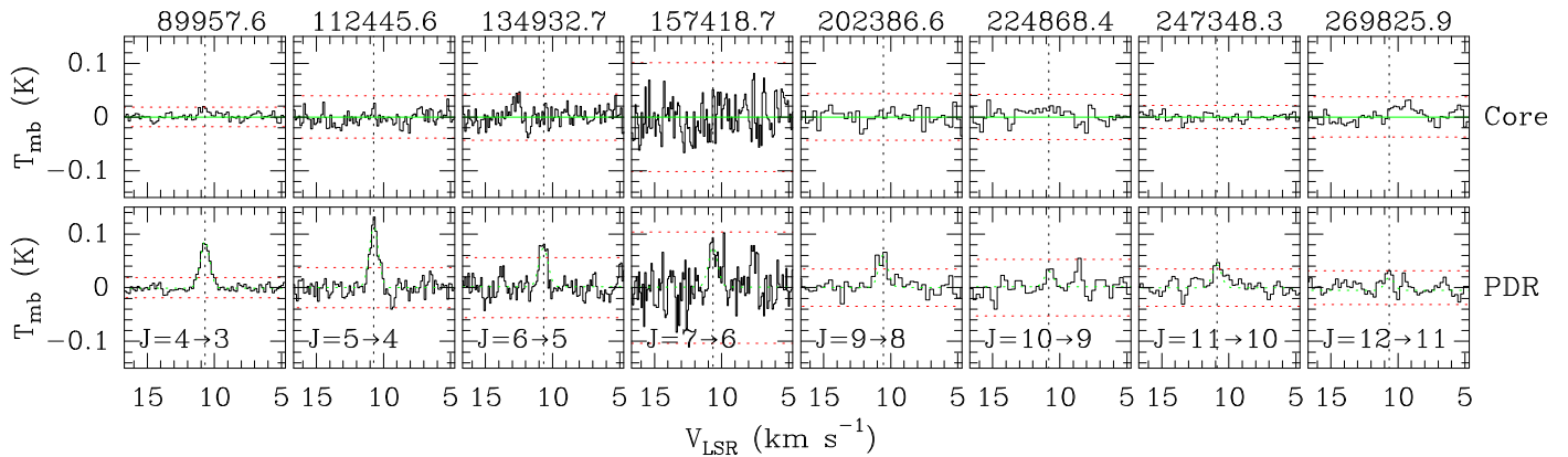
Fig. 1. Millimeter lines attributed to the \text{l-C}_3\text{H}^+ cation in the PDR (lower panels) and the dense core (upper panels) positions. The numbers above each panel are the line rest frequencies in MHz. The spectra and the Gaussian fits are shown as black histograms and green curves, respectively. The inferred rest frequencies are displayed as vertical dotted black lines for v_{\text{lsr}} = 10.7 \text{ km s}^{-1} and \pm 3\sigma noise levels as horizontal dotted red lines.
