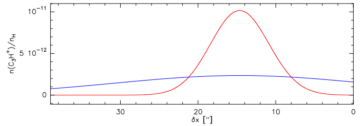
Fig. 6. Spatial profiles of the predicted abundance of C 3 H + cation. The modeled abundance profile was convolved along the x -axis with a Gaussian of 6''-FWHM (red line), and 27''-FWHM (blue line).
