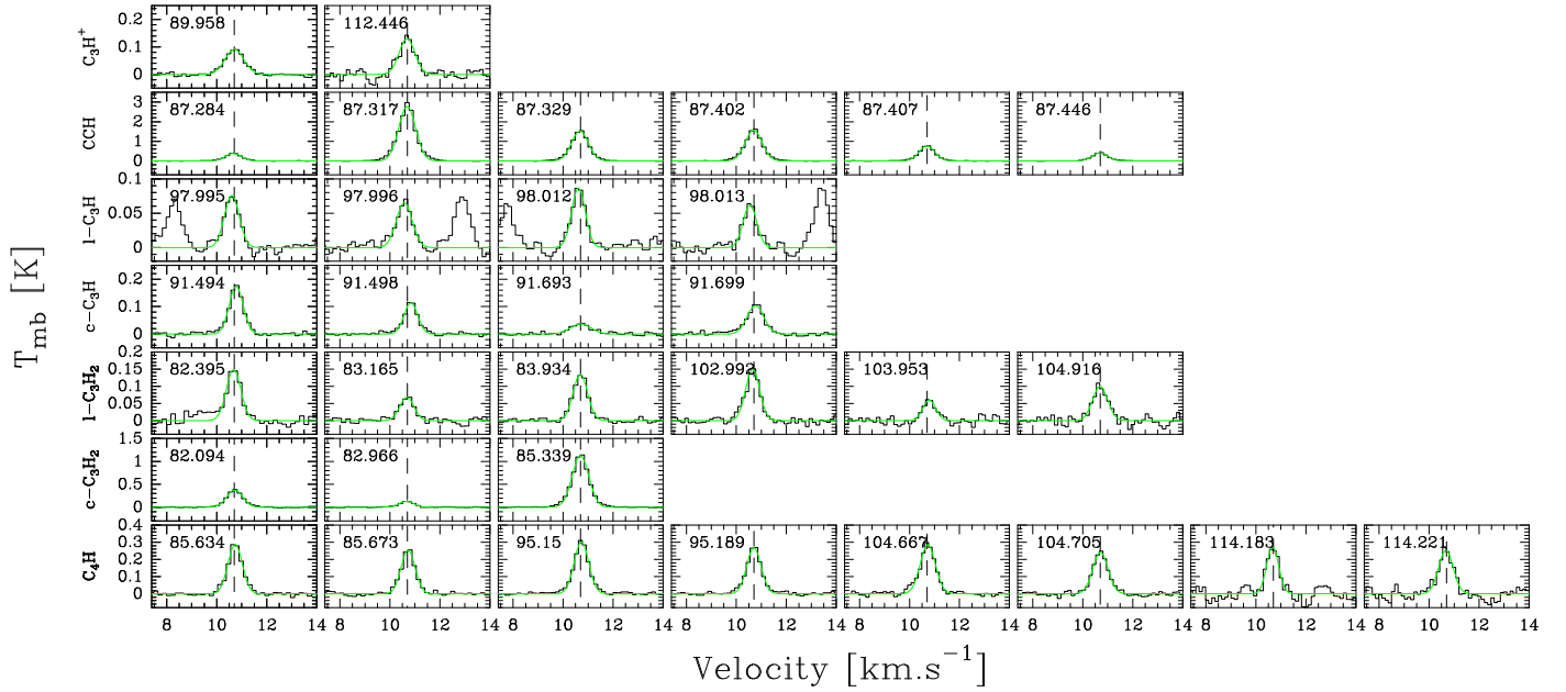
Fig. A.1. Hydrocarbon lines detected toward the Horsehead PDR at RA=5h40m53.936s, Dec=-2°28′00″ (J2000). Only lines in the 3 mm band, whose energy of the upper level is lower than 100 K and which have a higher signal-to-noise ratio than 8, are shown. The green lines are Gaussian fits. The vertical dashed lines mark 10.7 km s -1 .
