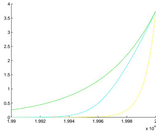
Figure 3.4: The curve in the middle represents C_{1000}^3 on [0.99L, L] . The upper curve represents the upperbound f for C^3 found in Lemma 3.4.2 and the the lower curve represents g , the bound from below.
