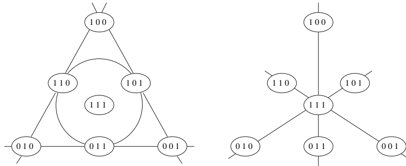
FIGURE 3. The algebras Cl_3 and \mathbb{M}_3 .
