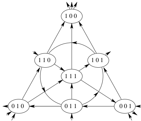
FIGURE 1. (\mathbb{Z}_2)^3 -grading on the octonions.
