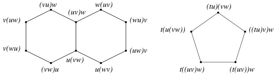
FIGURE 2. Two hexagonal and the pentagonal commutative diagrams
