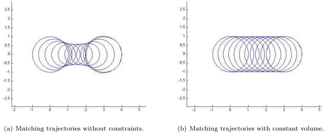
Figure 1: Matching trajectories.
