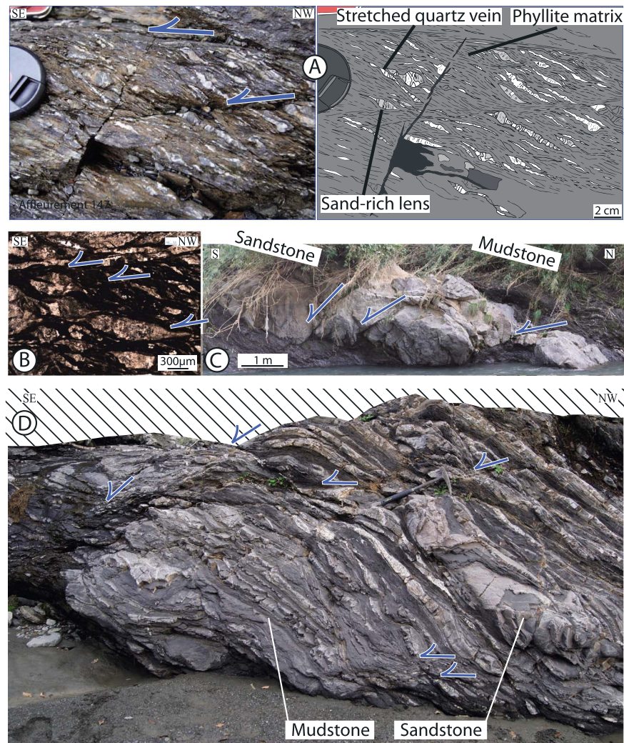
Figure 7. D3 deformation stage with the top-to-the-SE simple shear kinematics. (a and b) The top-to-the-SE shear zones, pervasive throughout the Hyuga Mélange unit, deform asymmetrically the centimeter- to millimeter-scale blocks of sandstones (light gray in Figure 7a, right) embedded in the phyllitic matrix (dark gray). Note the ubiquitous fragments of quartz veins (white), either cutting across sandstone blocks or as blocks in the matrix. (c and d) The top-to-the-SE faults and shear bands are also present in the structurally lower Coherent Hyuga, offsetting a large sandstone boudin surrounded by mudstone richer layers (Figure 7c) or alternating sandstone and mudstone beds (Figure 7d).
