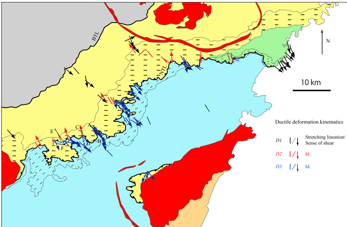
Figure 3. Ductile deformation map (see location in Figure 1). Nonnarrowed rods indicate coaxial stretching; arrows indicate asymmetrical simple shear (e.g., arrows pointing to the north represent a top-to-the-north sense of shear). Deformation microstructures have been assigned to the tectonic stages defined in the text.
