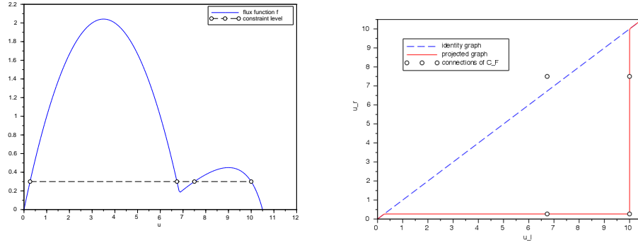
Fig. 1. Example of §4.5. The flux function f , represented in the left figure, is not a bell-shaped function. Therefore, the set \mathfrak{C}_F contains 4 singletons represented in the right figure by black circles. The graph \beta (red solid line) is defined as the projection of the identity (blue dashed line) on the set of the maximal monotone graphs containing the strict connections of \mathfrak{C}_F located below the graph Id.
