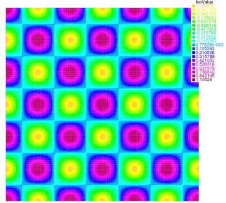
FIGURE 2. Exact pressure
