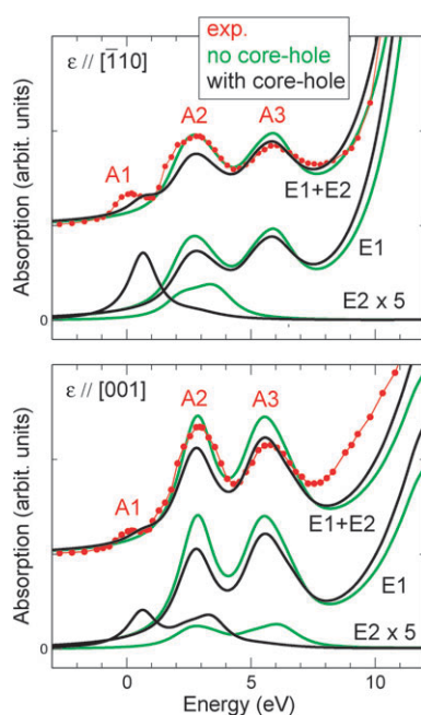
Fig. 3 Comparison between experimental (red line with circles) and calculated (solid line) Ti K pre-edge spectra of rutile, for the \hat{\epsilon} \parallel z (bottom) and \hat{\epsilon} \perp z (top) experimental configurations. The theoretical spectra were calculated for a supercell including a core-hole (black line) or not (green lines), in order to show the effects of the presence of the 1s core-hole. The zero energy corresponds to the highest occupied state of the calculation including the core-hole effects. Note that the E2 contribution has been multiplied by 5 for clarity.
