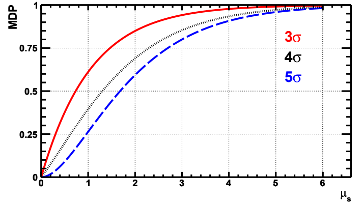
Fig. 6. Model discovery potential MDP versus number of signal events \mu_s for 3\sigma (red solid line), 4\sigma (black dotted), and 5\sigma (blue dashed) for GRB 110918.
