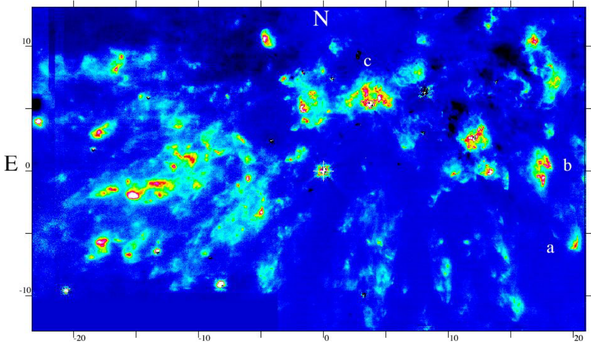
Fig. 1. H_2 emission in the 1–0 S(1) line at 2.121 \mu\text{m} , with continuum emission subtracted. Image size: 44.5'' \times 26'' . The cross indicates the position of the star TCC016 ( 05^{\text{h}}35^{\text{m}}14^{\text{s}}.91 , -05^{\circ}22'39''.31 (J2000)) and a,b,c identify objects shown in more detail in subsequents. The SE and ESE frames, referred to in the text, are respectively the regions to the west and to the east of TCC0016.
