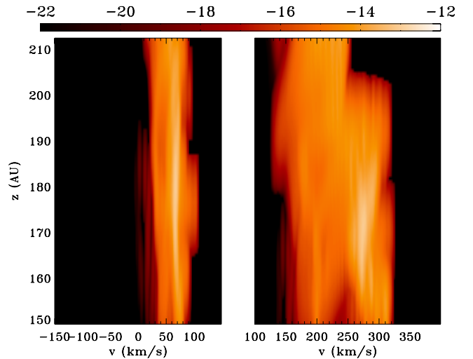
Fig. 10. Position–velocity diagrams for a declination angle with the line of sight of 80^\circ (left) and 45^\circ (right), for the forbidden doublet of [S II]. Units in \text{erg cm}^{-2} \text{arcsec}^{-2} \text{s}^{-1} .
