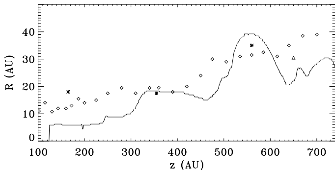
Fig. 11. Jet radius (solid line), R , as computed from the average of the doublets O I, N II, and S II for t = 21.6 . Diamonds denote observations of RW Aur, stars of HH 30, and triangles of HL Tau.
