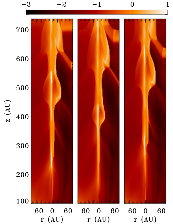
Fig. 4. Logarithmic maps of the density in normalized units of 10^4 \text{ cm}^{-3} (left axis of each panel), and the temperature in 10^4 \text{ K} (right axis of each panel), for the model employing the MINEq cooling. From left to right , three moments of the temporal evolution are shown, i.e., 16.8, 19.2, and 21.6 years. The jet is propagating upward, and specifically, the high density region located between 200 and 300 AU in the left panel , is found between 400 and 500 AU in the middle , and between 600 and 700 AU in the right panel .
