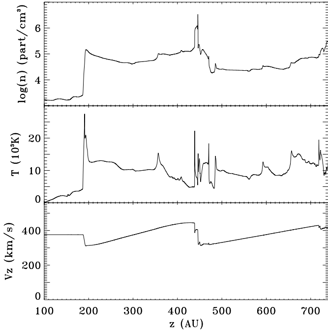
Fig. 2. Logarithmic number density ( top ), temperature ( middle ), and velocity ( bottom ) profiles along the axis, for the model adopting SNEq. The jet is moving from left to right and the displayed moment corresponds to t = 12 yr.
