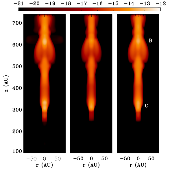
Fig. 9. Logarithmic maps of the surface brightness, processed as described in Fig. 7, for the three forbidden doublets of [O I], [N II], and [S II] (from left to right), in units of \text{erg cm}^{-2} \text{arcsec}^{-2} \text{s}^{-1} . The snapshot corresponds to t = 21.6 yr.
