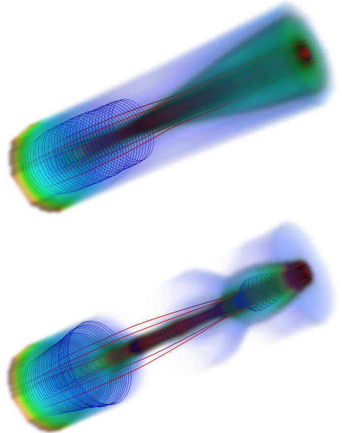
Fig. 1. 3D representation of the density distribution of the initial conditions ( top ) and at a later time during evolution ( bottom ). Blue/red corresponds to low/high density, the thin blue lines denote the magnetic field and the thick red lines the flow.
