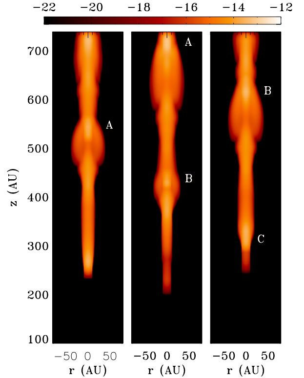
Fig. 7. Logarithmic maps of the surface brightness of the forbidden doublet [S II], convolved with the PSF, for the three moments shown in Fig. 4. The image is in units of \text{erg cm}^{-2} \text{arcsec}^{-2} \text{s}^{-1} and has been projected with a declination angle of 80^\circ with respect to the line of sight. The knots are labeled with letters.
