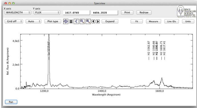
Figure 6: Example of 1D spectrum plotted with Specview. Several theoretical lines have been retrieved and plotted on the top of the investigated spectrum through the button "Lines IDs": the H-Ly \alpha line is provided by default with Specview, while the H 2 lines have been retrieved from the SESAM catalog.
