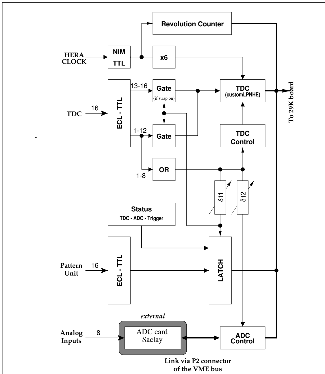
Figure 5: The L0 VME card
