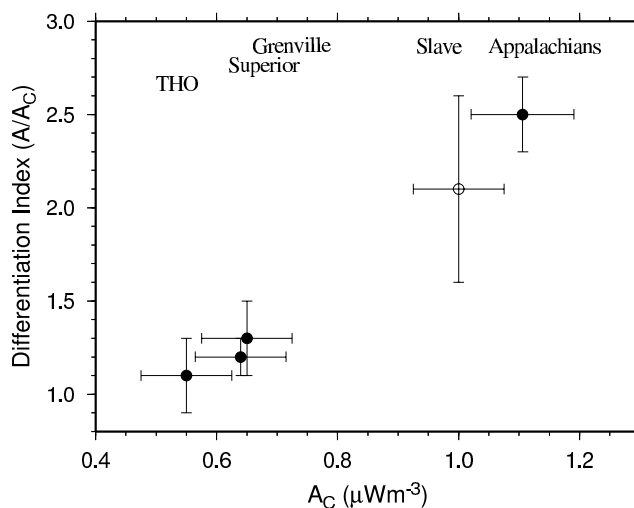
Figure 12. Differentiation index of crustal rocks ( \bar{A}/A_c ), where \bar{A} is the surface-averaged heat production and A_c is the bulk average heat production, as a function of the bulk average heat production. The Slave Province calculation is represented by an open circle since the heat flow data set is small compared to those in the other provinces. Error bars associated with D_i and A_c were calculated assuming a wide range for Moho heat flow between 12 \leq Q_M \leq 18 \text{ mW m}^{-2} .
