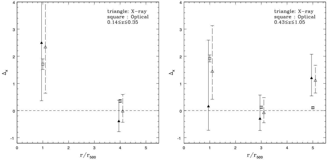
Fig. 8. Spatial stacked optical galaxy (open squares) and X-ray point source overdensities as a function of projected radial distance from the center of the cluster, including only clusters in the CFHTLS region (solid triangles) and including clusters in the CFHT ABC supplementary pointings (dashed triangles). Left panel: the low- z cluster sample. Right panel: the high- z cluster sample. Uncertainties are Poisson 1\sigma errors for small numbers (Gehrels 1986).
