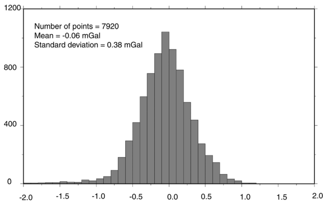
Figure 7. Histogram of residuals on the gravity anomaly (initial data from KMS 2002 satellite-derived gravity anomalies minus approximated data from 9651 wavelet representation) at 35 km resolution.
