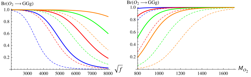
Fig. 1. The dependence of the branching ratio of the decay of a light sgluon to two gravitinos and a gluon on the SUSY breaking scale (left plot) and the mass of the light sgluon (right plot). Full lines are drawn for \delta\tilde{m} = M_Z = 90 GeV and dotted lines for \delta\tilde{m} = 180 GeV. Also, we have taken m_{\tilde{g}} = 1.7 TeV and m_{\tilde{q}} = 1.5 TeV. Left plot (blue, red, green, orange): M_{O_2} = (0.8 TeV, 1 TeV, 1.2 TeV, 1.4 TeV). Right plot (blue, red, green, orange): \sqrt{f} = (3 TeV, 4 TeV, 5 TeV, 6 TeV). (For interpretation of the references to colour in this figure legend, the reader is referred to the web version of this article.)
