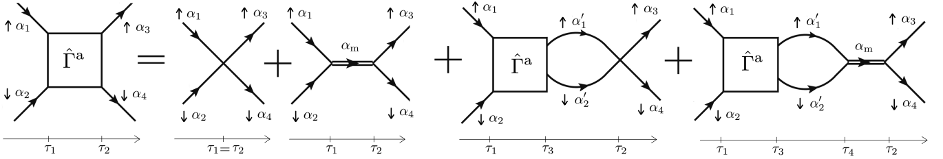
FIG. 3: Diagrammatic form of the Bethe-Salpeter equation for the atom-atom vertex \hat{\Gamma}^a .
