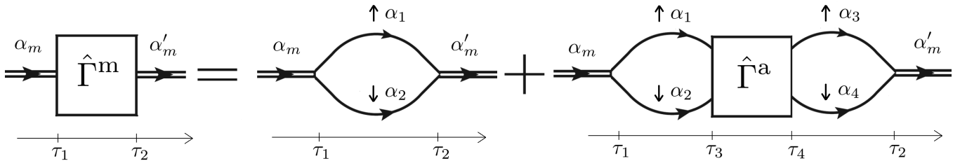
FIG. 4: Diagrammatic form of Eq. (95).
