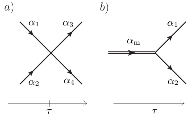
FIG. 2: a) Vertex associated with the direct interaction in the finite-temperature formalism : g \langle \alpha_1 \alpha_2 | \hat{A}_\epsilon^\dagger \hat{A}_\epsilon | \alpha_3 \alpha_4 \rangle \delta(\tau) ; b) idem for the interchannel coupling : \Lambda \langle \alpha_m | \hat{A}_\epsilon | \alpha_1 \alpha_2 \rangle \delta(\tau) .
