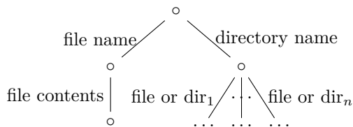
Figure 3: File system as a data tree.
