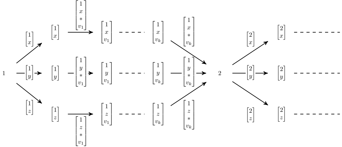
Figure 6: Automaton H_1 .
