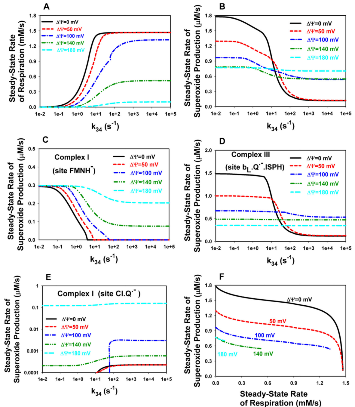
Fig. 6. Computer simulated partial inhibition of the \text{O}_2^- production rate by antimycin A (A–E) Steady state dependency of the rates of respiration (A), total \text{O}_2^- production by Complexes I and III (B), \text{O}_2^- production by the reduced flavin of Complex I (C), the unstable semiquinone of Complex III (D), and the semiquinone of Complex I (E) on the rate constant k_{34} at different values of \Psi .
