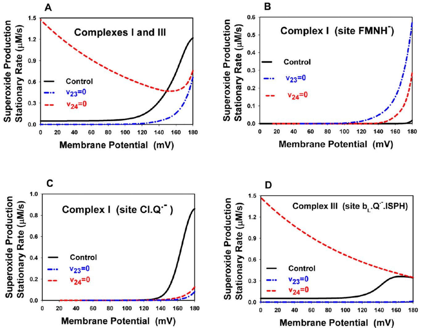
Fig. 7. Computer simulated effect of inhibition of different reactions at the Qo site on the O_2^{\cdot-} production rate during oxidation of succinate alone (A–D) The computer simulated O_2^{\cdot-} production rate upon inhibition of the first ( v_{23}=0 ) or the second ( v_{24}=0 ) electron transfer in the Qo site of Complex III. (A) The total rate of O_2^{\cdot-} generation by both Complexes I and III. (B–D) The rate of O_2^{\cdot-} generation by different sites of Complexes I and III: (B) the site FMNH - of Complex I; (C) the semiquinone of Complex I (complex Cl.Q - ); (D) the unstable semiquinone of Complex III (complex b L .Q - .ISPH). All computer simulations were performed using model E. Values of all parameters in the control model E are the same as for Fig. 5. Black solid curves correspond to the computer simulated O_2^{\cdot-} production rate in the control model E. Blue dash-dot and red dashed curves are the O_2^{\cdot-} production rates in the same model E, except for the rates v_{23} and v_{24} which were taken to be 0 to simulate the effects of stigmatellin or myxothiazol. Succinate alone was modeled as a respiratory substrate ( V_{\max 19} = 4270 \mu\text{M/s} ; k_{15} = 0 ).
