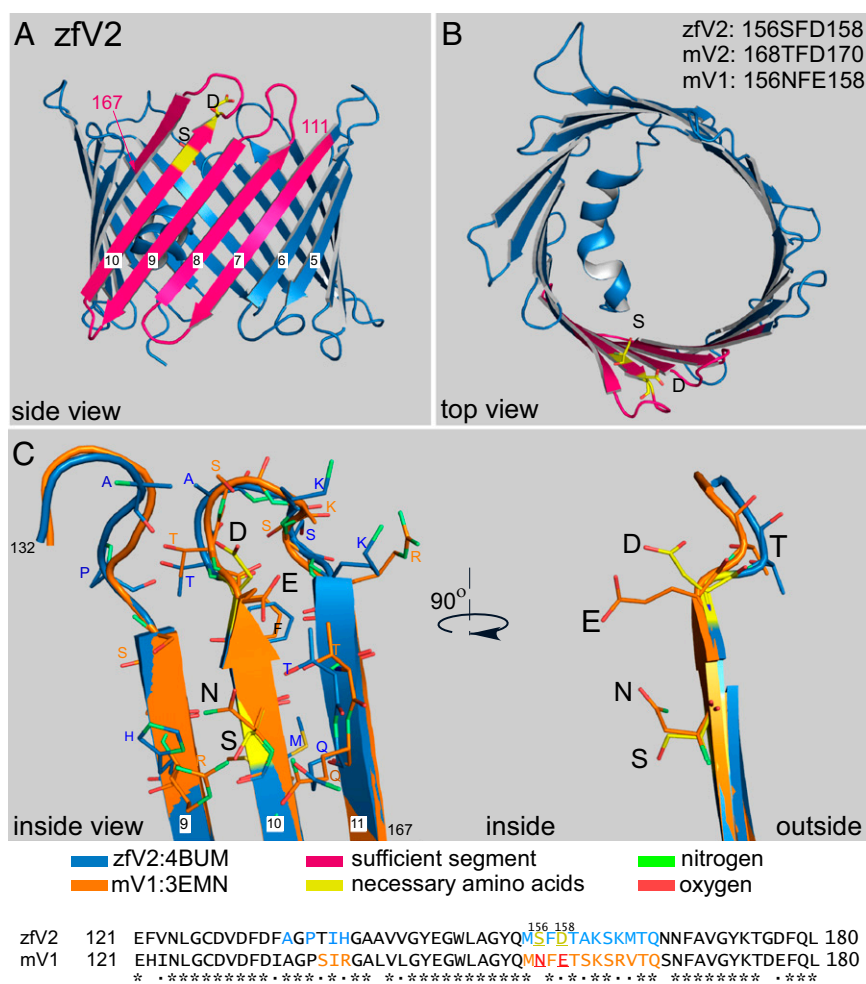
Fig. 6. Three-dimensional structure of zfV2. ( A and B ) Side and top views of zfV2 (PDB ID code 4bum) illustrated using Pymol. Pink is the sufficient segment, and yellow (sticks) is the necessary residues, including S156 and D158. ( C, Right ) Side view of the segment containing amino acids S156 and D158 (yellow sticks) in zfV2 vs. the relevant residues in mV1 (N156 and E158, orange sticks). Residues 111–167 in zfV2 (blue) and mV1 (PDB ID code: 3emn, orange) were superimposed. ( C, Left ) Interior view of the channels showing the residues that are within a distance of 4 Å from either S156 or D158 in zfV2 (sticks with carbon colored blue) or N156 or E158 in V1 (sticks with carbon colored orange). In sticks, oxygen is red and nitrogen is green. Adjacent residues have also been marked in the sequences of zfV2 (blue) and mV1 (orange).
