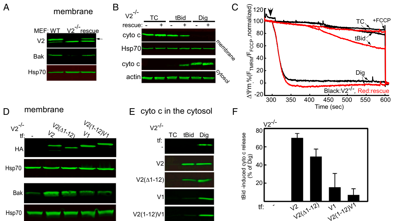
Fig. 1. Genetic rescue studies in V2 -/- MEFs. Unique N-terminal extension in V2 is neither necessary nor enough for Bak import and cyto c release. (A) Western blot verification of the presence of V2 and Bak in the membrane fraction of WT and V2 -/- cells rescued with avV2. The arrow shows the relevant band of V2. (B) Cyto c release was monitored by detecting the cyto c level in the membrane and cytosolic fraction of nonrescued (-) and avV2-rescued (+) V2 -/- permeabilized MEFs 5 min after treatment with solvent [tBid (25 nM) or digitonin (Dig, 600 \mu g/mL)]. TC, time control. Hsp70 and actin were used as loading controls. (C) Representative traces for the time course of \Delta\Psi_m recorded in cell suspensions using a fluorometer. The experiment was carried out in permeabilized V2 -/- (black line) or avV2-rescued V2 -/- (red line) cells treated with tBid or Dig (added at 300 s, marked by an arrow). FCCP (5 \mu M) was added at the end of the recordings to dissipate the remaining \Delta\Psi_m . Data are presented as the percentage of the initial \Delta\Psi_m . TCs are the nontreated samples. (D) HA and Bak Western blot of the membrane fraction of V2 -/- cells transfected (tf) with HA-tagged V2, V2( \Delta 1-12), V1, or V2(1-12)V1. Immunoblot (E) and quantitative analysis (F) of cyto c in the cytosolic fraction of V2 -/- cells transfected with V2, V2( \Delta 1-12), V1, or V2(1-12)V1 and treated with tBid or Dig after plasma membrane permeabilization. In response to tBid, the cyto c band was normalized to the response to Dig in each condition ( n = 3 ).
