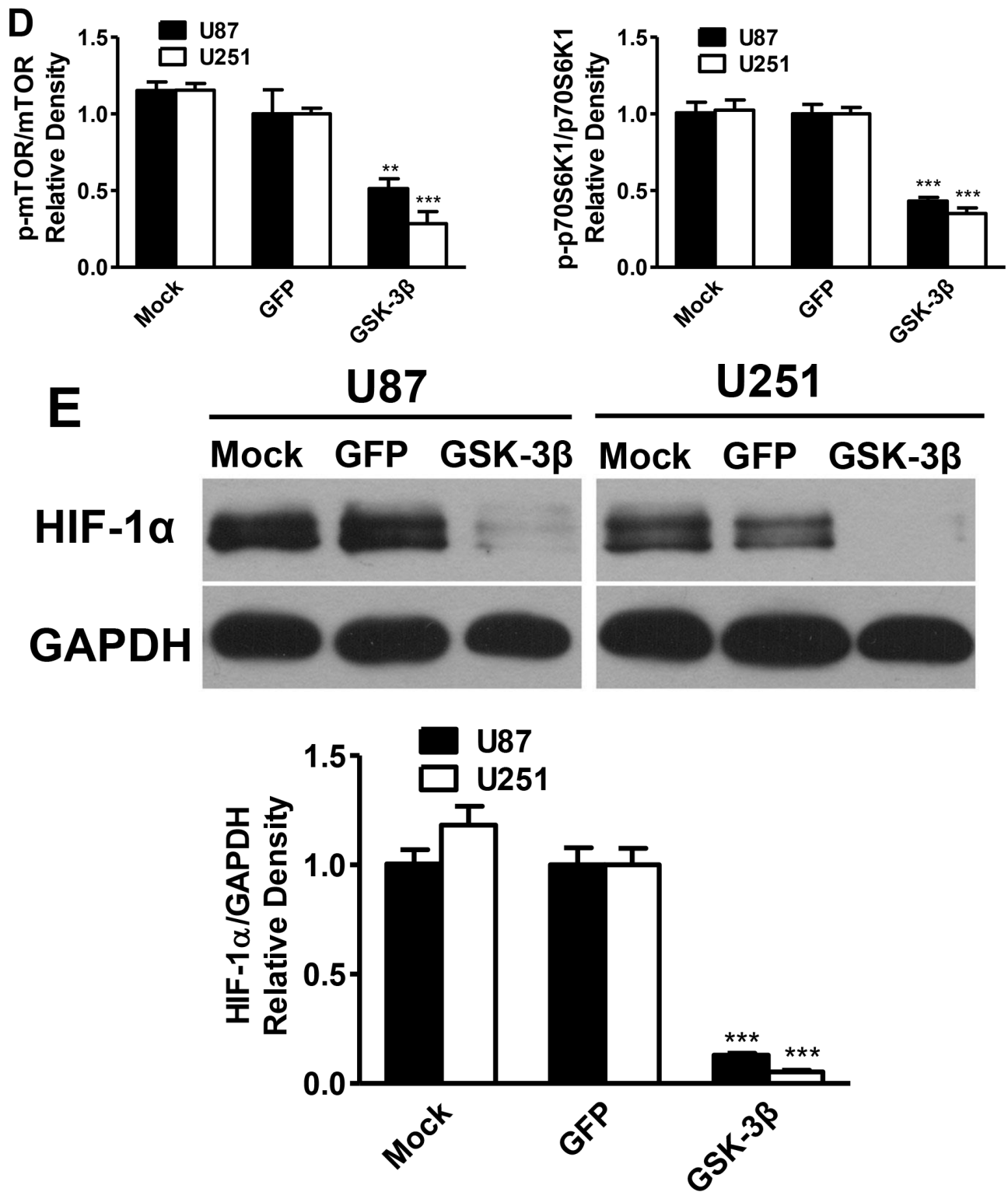
Figure 2: (Continued) Overexpression of GSK-3β attenuated β-catenin and mTOR/p70S6K1 activation in human glioma cells. D. and E. Cells transfected with or without adenovirus carrying GSK-3β or GFP were subjected to Western blotting analysis for mTOR, p-mTOR, p70S6K1, p-p70S6K1, HIF-1α and GAPDH expression. The protein levels from three independent experiments are quantified and presented as mean ± SD. Asterisk indicates significant difference when compared to the control ( P < 0.05 ). (Continued)
