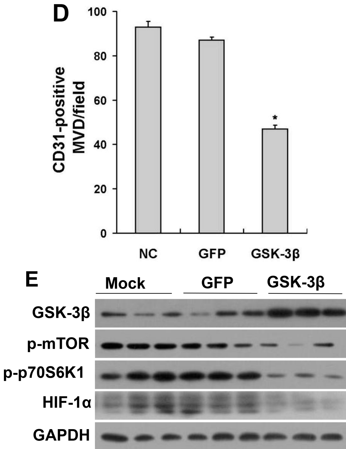
Figure 4: (Continued) Overexpression of GSK-3 \beta decreased tumor growth in vivo . D. Quantitative analysis of MVD in the xenograft plugs sections. The graph represents the mean \pm SD from five different tumor sections for each group. *indicated significant difference at p < 0.05 . E. The protein levels of mTOR, p-mTOR, p70S6K1, p-p70S6K1 and HIF-1 \alpha in tumor tissues were analyzed by Western blotting. GAPDH was used as internal control. (Continued)
