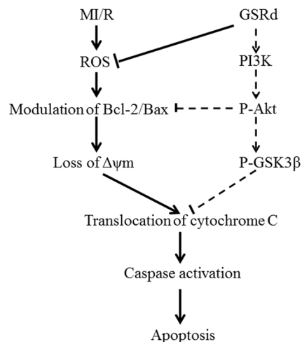
Figure 9. Schematic diagram depicting protective signaling of GSRd in MI/R-induced apoptosis. GSRd inhibits the apoptotic signaling cascades initiated by MI/R-generated ROS. Arrows (→) indicate activation or induction, and segments ending with a (⊥) indicate inhibition/blockade. Solid lines (—) indicate mechanisms strongly supported by the current study, and dotted lines (---) indicate hypothesized connections requiring further investigations. doi:10.1371/journal.pone.0070956.g009
