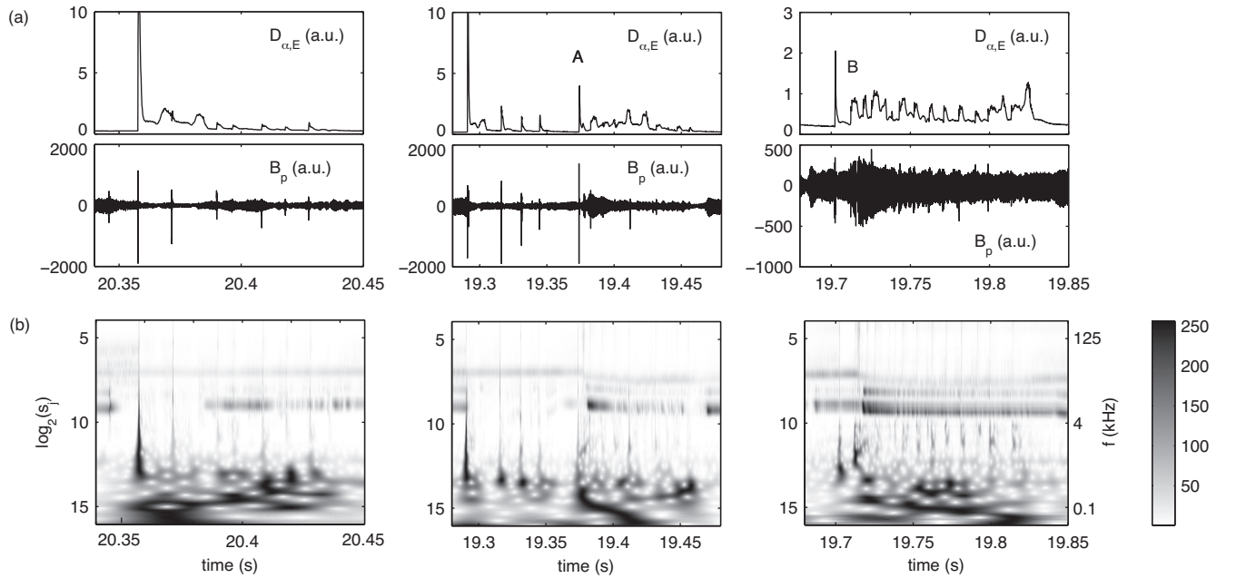
Figure 5. JPN 59423. (a) time trace of D_{\alpha,E} measured in the divertor region, and of \dot{B}_p measured on the outboard plane, in the case of spontaneous compound ELMs (left), pellet A (center) and pellet B (right). (b) Wavelet scalogram computed in the same time windows. The sawtooth precursors with n=1,2 and the NTM are visible in the wavelet scalogram.
