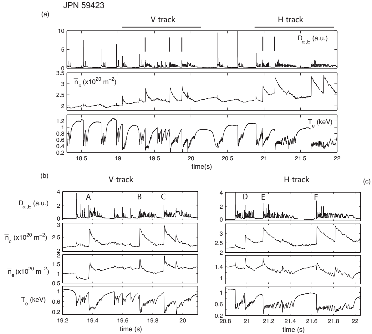
Figure 2. JPN 59423: B_T = 2.4 T, I_P = 2.5 MA, P_{NBI} = 15 MW, P_{RF} = 3 MW. (a) Time traces of the D_\alpha emission measured in the inner divertor, of the line integrated electron density measured through a line sight intersecting the plasma axis \bar{n}_{e,c} and of the electron temperature T_e measured inside the edge transport barrier, in the pedestal region. Vertical lines in the top plot indicate pellets that are not fragmented. (b) extended view over the time window where pellets are injected from the top (vertical track). (c) extended view over the time window where pellets are injected from the high field side (inboard track). The line integrated density measured at the edge, \bar{n}_e , is shown in (b) and (c) for comparison. A-E indicate pellet-triggered events, F indicate a spontaneous ELM almost synchronous with the injection of a pellet.
