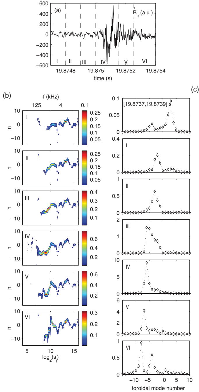
Figure 8. (Colour online) JPN 59423, pellet C. (a) time trace of magnetic perturbations \hat{B}_p of the pELM triggered by event C. (b) Scale dependent toroidal mode number spectrum P(n, s) , computed over the time windows I-VI, as indicated in (a). (c) Toroidal mode number spectrum, P(n) , obtained integrating P(n, s) over scales \log_2(s_j) = [4, 10] . For comparison it is also shown P(n) computed 1 ms before the pELM crash (top frame).
