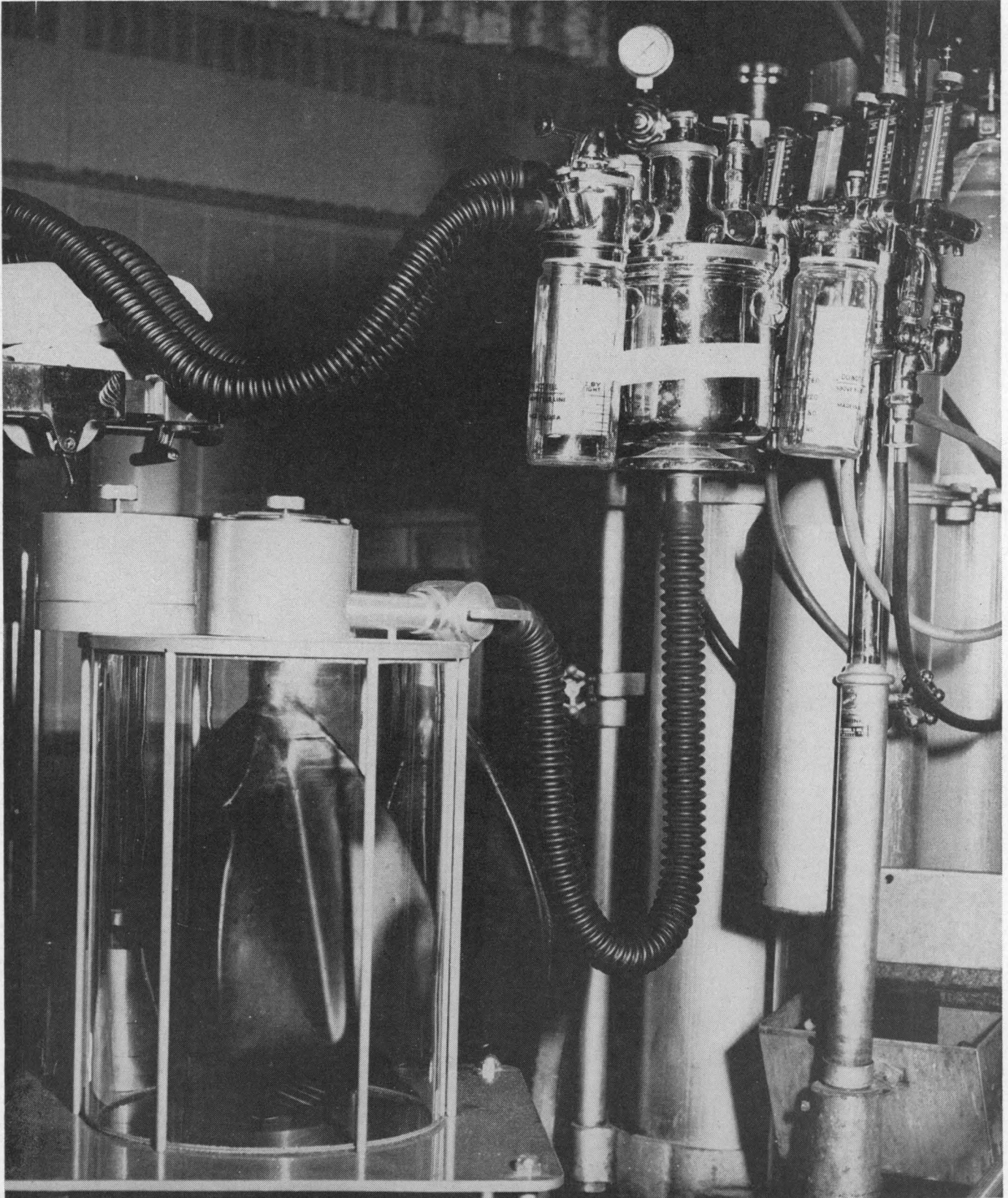
The Jefferson Ventilator in use with a standard anesthesia apparatus. Readily controllable positive and negative pressures are applied to adequately ventilate the anesthetized patient.
