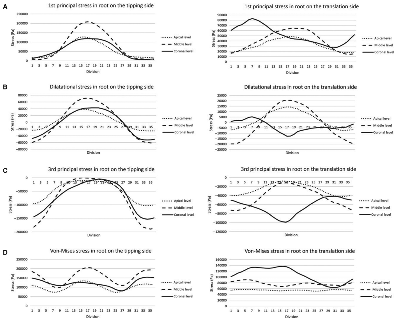
Fig. 3. Stress invariant distributions at the root surfaces in the 3 by 36 root surface divisions corresponding to two treatment strategies, tipping and translation, 1st principal stress (a), dilatational stress (b), 3rd principal stress (c), and von Mises stress (d).
