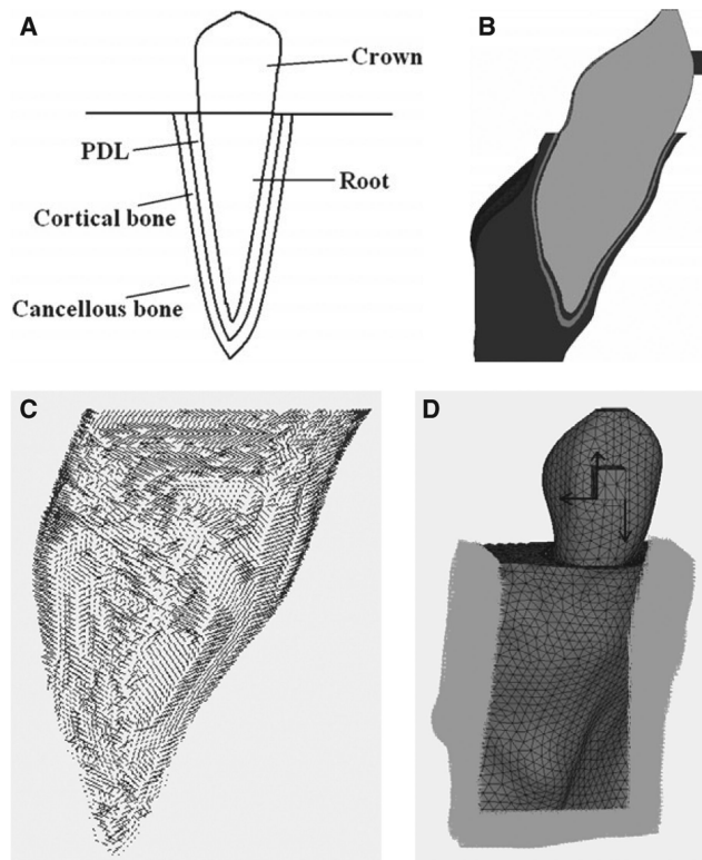
Fig. 1. (A) Schematic diagram of the FE model, (B) Tooth–PDL–bone–bracket model, (C) PDL fiber model, and (D) mesh and boundary/loading conditions. FE, finite element; PDL, periodontal ligament.
