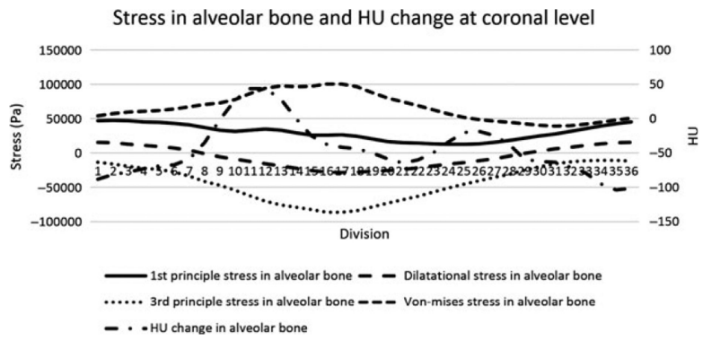
Fig. 6. Comparison of stresses and Hounsfield Unit (HU) change in the 36 alveolar bone divisions at the coronal level. High dilatational stress area in the bone in the direction of tooth movement and low in the opposite direction had high HU reduction, indicating high remodeling.
