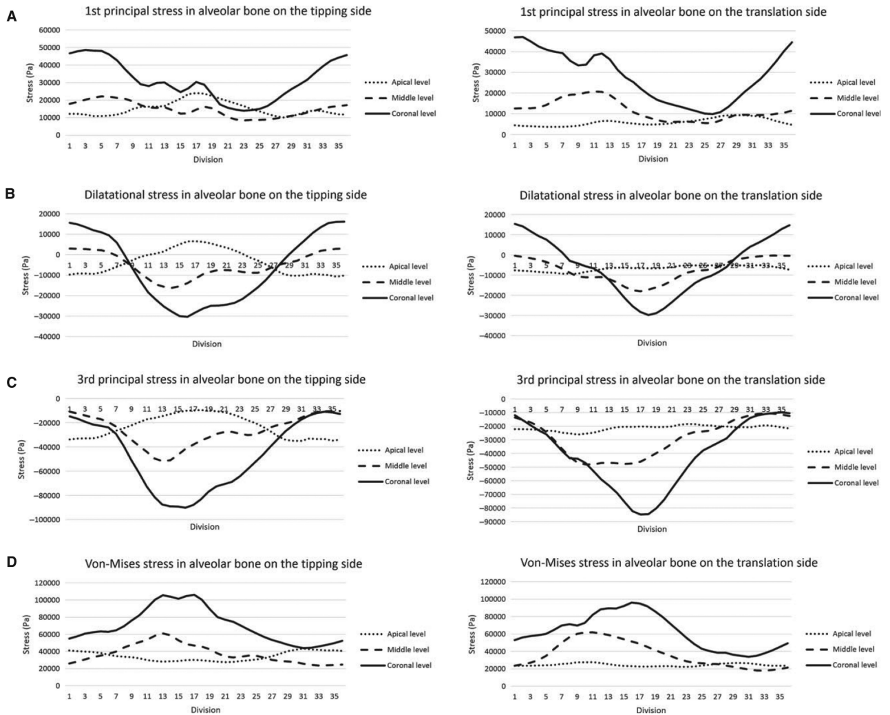
Fig. 5. Stress invariant distributions in the 3 by 36 bone divisions corresponding to two treatment strategies, tipping and translation 1st principal stress (a), dilatational stress (b), 3rd principal stress (c), and von Mises stress (d).
