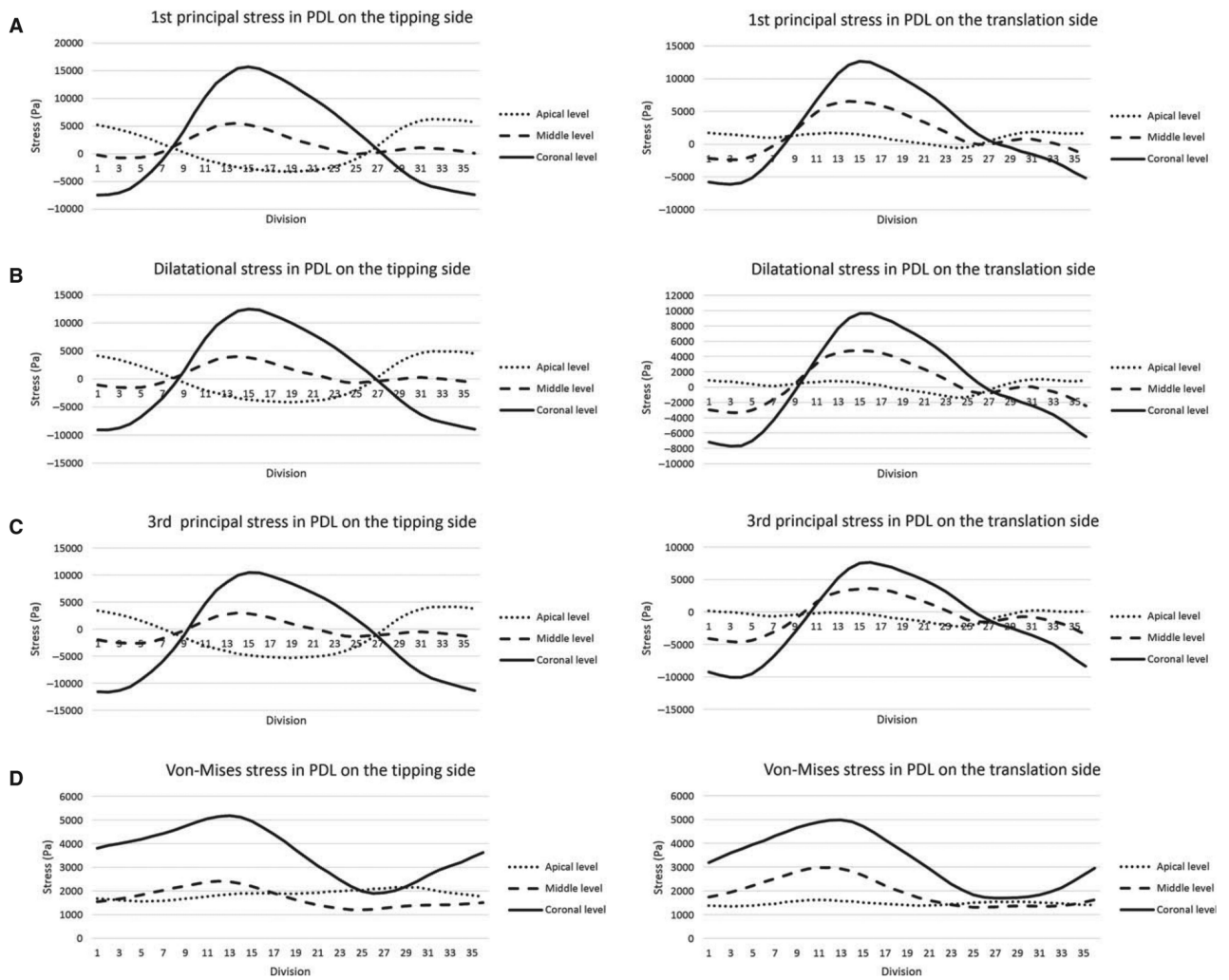
Fig. 4. Stress invariant distributions in the 3 by 36 PDL divisions corresponding to two treatment strategies, tipping and translation, 1st principal stress (a), dilatational stress (b), 3rd principal stress (c), and von Mises stress (d). PDL, periodontal ligament.
