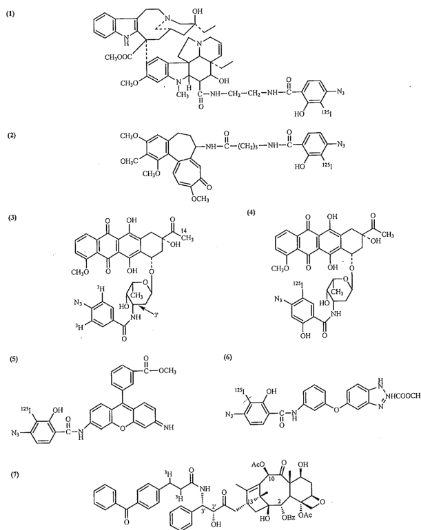
Fig. (1). Structures of photoaffinity analogs of MDR-related drugs known to covalently label P-glycoprotein: (1) [^{125}\text{I}]\text{NASV} , (2) [^{125}\text{I}]\text{NASC} , (3) [^3\text{H}]\text{NAB-DNR} , (4) [^{125}\text{I}]\text{NAS-DNR} , (5) [^{125}\text{I}]\text{ASA-Rh123} , (6) [^{125}\text{I}]\text{ASA-BZ} , and (7) [^3\text{H}]\text{BzDC-paclitaxel} .
