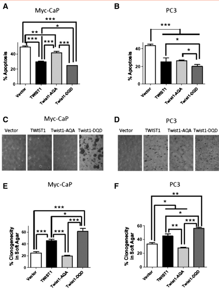
Figure 4. The Twist1-AQA mutant is defective for TWIST1-induced soft agar tumorigenicity. Cells were grown adherent or in suspension using ultra-low attachment dishes. The amount of apoptotic cell death or anoikis for the ultra-low attachment conditions was quantified by Annexin V–Alexa Fluor 488 and PI staining followed by flow cytometric analysis. Percent apoptosis was calculated by normalizing total apoptotic fraction in ultra-low attachment conditions to that of adherent cells and plotted as bar graph \pm SEM for (A) Myc-CaP ( n = 7 ) and (B) PC3 ( n = 6 ) TWIST1 isogenic cell lines ( *P < .05 , **P < .01 , and ***P < .001 by paired two-tailed t test); 5 \times 10^5 cells were embedded in soft agar and incubated for 2 weeks. Colonies containing more than 50 cells were scored in at least five random fields. Representative phase contrast images of (C) Myc-CaP and (D) PC3 TWIST1 isogenic cell lines at \times 4 magnification are shown. The percent clonogenicity in soft agar is calculated by normalizing the number of colonies to the total number of cells and represented as bar graphs \pm SEM for (E) Myc-CaP ( n = 6 ) and (F) PC3 ( n = 6 ) ( *P < .05 , **P < .01 , and ***P < .0001 by Mann-Whitney test).
