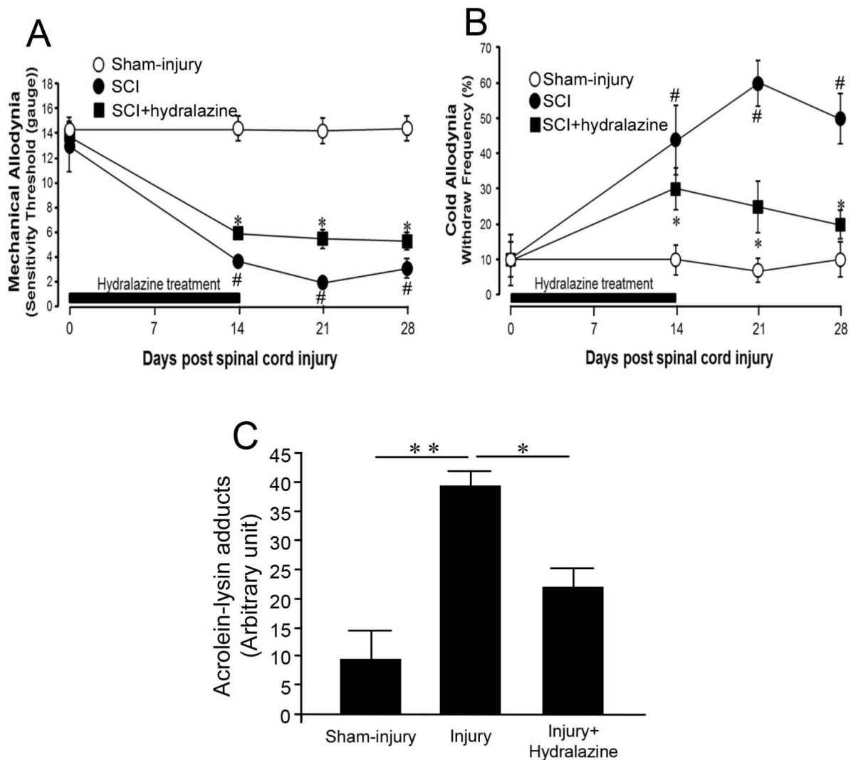
Figure 5. Daily hydalazine injections for fourteen days after thoracic spinal cord injury (SCI) attenuate behavioral changes in response to mechanical and cold stimuli for at least 28 days. At day 0, before SCI, there was no difference in mechanical and cold hyperreflexia assessments in sham injured control, SCI alone, and SCI in combination with hydalazine. However, on days 14-28 post injury, SCI alone rats displayed a significantly increased level of both mechanical and cold hyperreflexia. (A-B, # P < 0.05 when compared to the sham injured control). This increased display of presumptive pain behavior was significantly attenuated with the addition of hydalazine (* P < 0.05 when compared to SCI alone). C). Bar graph displaying the elevation of the acrolein-lysine adduct level and its attenuation by hydalazine one day after SCI. ( n=6 in each condition). (* P < 0.05 , ** P < 0.01 , ANOVA). All data (A-C) were expressed in mean \pm SEM.
