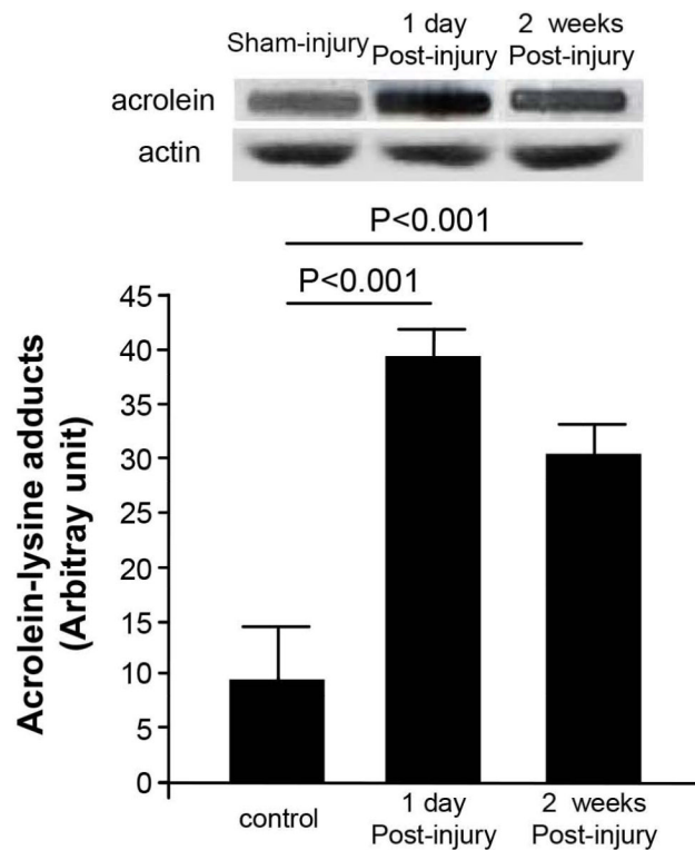
Figure 1. Persistent elevation of acrolein adducts following thoracic spinal cord injury (SCI) in rats. SCI induces acrolein elevation in spinal cord tissue associated with contused tissue for at least 2 weeks. Dot immunoblotting assay demonstrated that SCI acrolein lysine adduct levels were elevated as early as 24 hours after injury when compared with samples derived from sham injury animals at 1 day. These elevations were observed for at least 2 weeks after SCI. All data was expressed as mean \pm SEM. n=6 in all cases.
