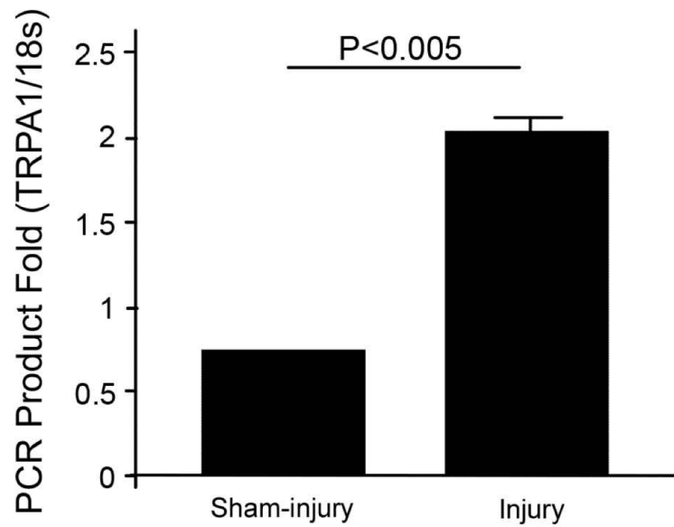
Figure 2. RT-PCR relative quantification of TRPA1 mRNA in lumbar (L3-6) dorsal root ganglia (DRG) 7 days after spinal cord injury (SCI). Gene expression was normalized by the expression of 18s and compared to the cycle threshold (Ct) value for 18s of SCI tissue mRNA. The difference of gene expression is shown as the fold ratio. Relative transcript level was calculated as X = 2^{-\Delta\Delta Ct} , where \Delta\Delta Ct = \Delta E - \Delta Ct and \Delta E = Ct_{exp} - Ct_{18s} , \Delta Ct = Ct_{control} - Ct_{18s} . There is a 2 fold increase in TRPA1 mRNA present seven days after SCI when compared to sham injury control group (n=4). For the statistical analysis, paired T-test was used (P<0.005).
