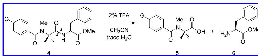
Scheme 2. Hydrolytic Instability of 4 as a Function of the Electronic Nature of G 6
