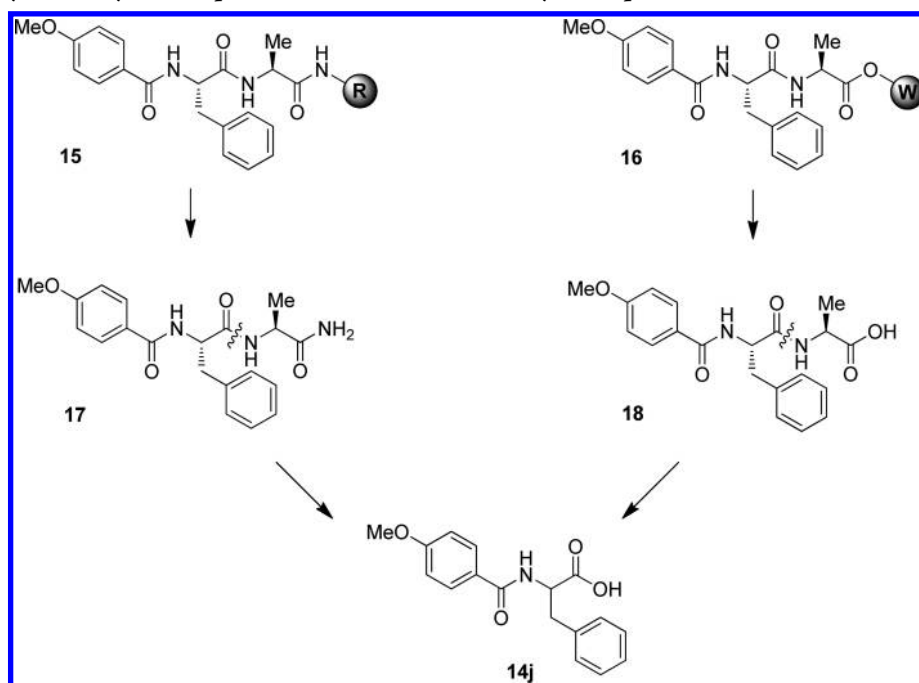
Scheme 5. Instability of N-Acylated Peptides as a Function of the Acyl Group
