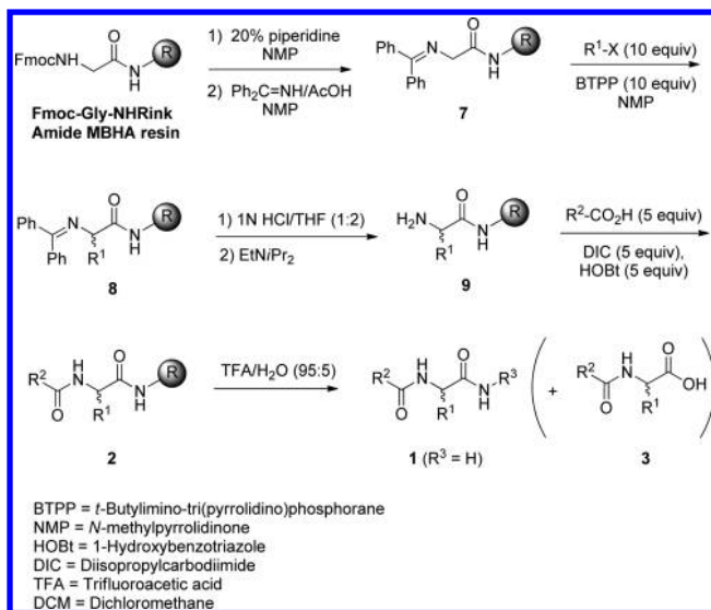
Scheme 3. Synthesis of N -Acylated Unnatural Amino Acid Amides 1 (R 3 = H)
