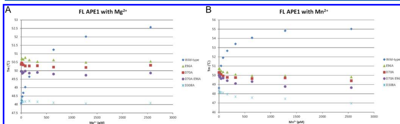
Figure 4. Effect of metal binding on the stability of wild-type, D70A, E96A, D70A/E96A, D308A, and full-length APE1. Differential scanning fluorimetry was used to measure the change in melting temperature, which is plotted versus the concentration of Mg^{2+} (A) or Mn^{2+} (B).
