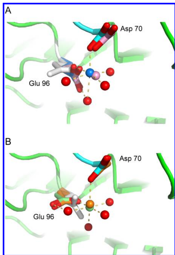
Figure 6. A comparison of coordinating ligands and distances for Mg^{2+} -bound APE1 structures. Two other structures from the PDB, 4LND (A) and 3U8U (B), are shown superimposed on our Mg^{2+} -APE1 structure. A cartoon rendering of our APE1 structure is shown in lime green. (A) The B conformation of E96 from our Mg^{2+} structure (marine blue) is in a similar conformation to that of E96 in 4LND (pink, oxygens in red). The A conformation of E96 is shown in gray. (B) The A conformation of E96 in our Mg^{2+} structure shown in lime green is in a similar conformation to that of E96 in 3U8U shown in orange; oxygens are shown in red. The B conformation of E96 is shown in gray. D70 is shown in a stick rendering with carbons in blue and oxygens in red for our structure, with carbons in pink for 4LND (A) and with carbons in orange for 3U8U (B). Bound Mg^{2+} for our structure is shown as a blue sphere in (A) and a green sphere in (B). Mg^{2+} in 4LND is shown as a pink sphere in (A) and in 3U8U is shown as an orange sphere in (B).
