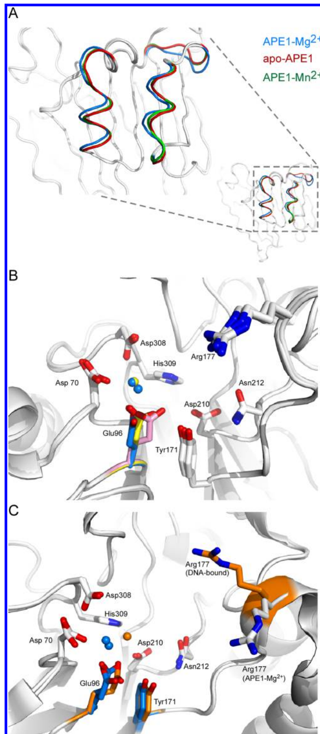
Figure 2. Structural comparisons are shown for different APE1 structures. (A) Differences between the \text{Mg}^{2+} -bound APE1 (blue ribbon rendering) and apo-APE1 (red) or \text{Mn}^{2+} -bound APE1 (green) structures are shown close-up and in the context of the full structure (inset) for the surface loop (amino acids 98–102) and two alpha helices (amino acids 77–86 and 106–113, respectively). Structural differences appear to correlate with the length of the b cell axis (Table 1), which is shorter in the \text{Mg}^{2+} -bound APE1 structure. (B) Active site residues are shown in stick renderings with carbons in gray, oxygens in red, and nitrogens in blue for superimposed structures of apo-APE1, APE1- \text{Mg}^{2+} , and APE1- \text{Mn}^{2+} . Overall, active site residues in each of the structures have a single conserved conformation including D210, N212, and H309 in all three structures. Small differences in the
