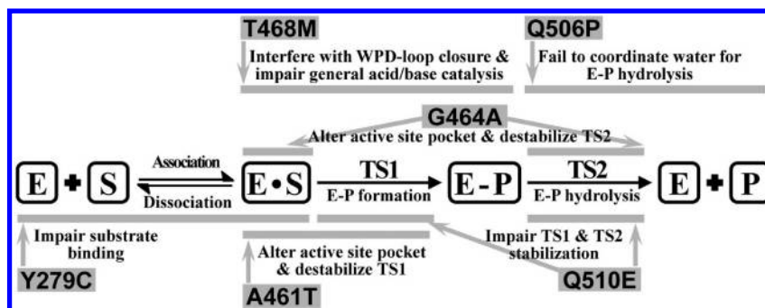
Figure 4. Schematic diagram showing the impact of LS-associated SHP2 mutations on the SHP2-catalyzed reaction.
