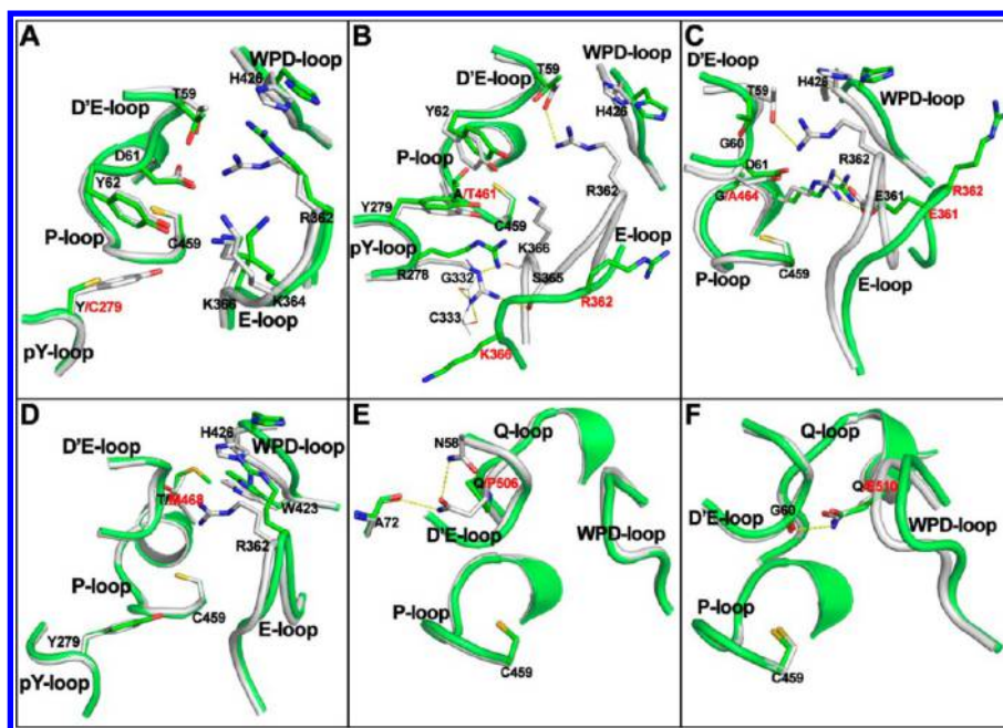
Figure 2. LS SHP2 mutation weakens the N-SH2–PTP interdomain interaction. The weakened interactions are represented by steric and/or electrostatic alterations within mutants (A) Y279C, (B) A461T, (C) G464A, (D) T468M, (E) Q506P, and (F) Q510E. In each panel, wild-type SHP2 is colored gray and the specific LS mutant green. The mutation site is colored red. Polar interactions that existed in the wild type but disappeared in the mutant are denoted with yellow dashed lines.
