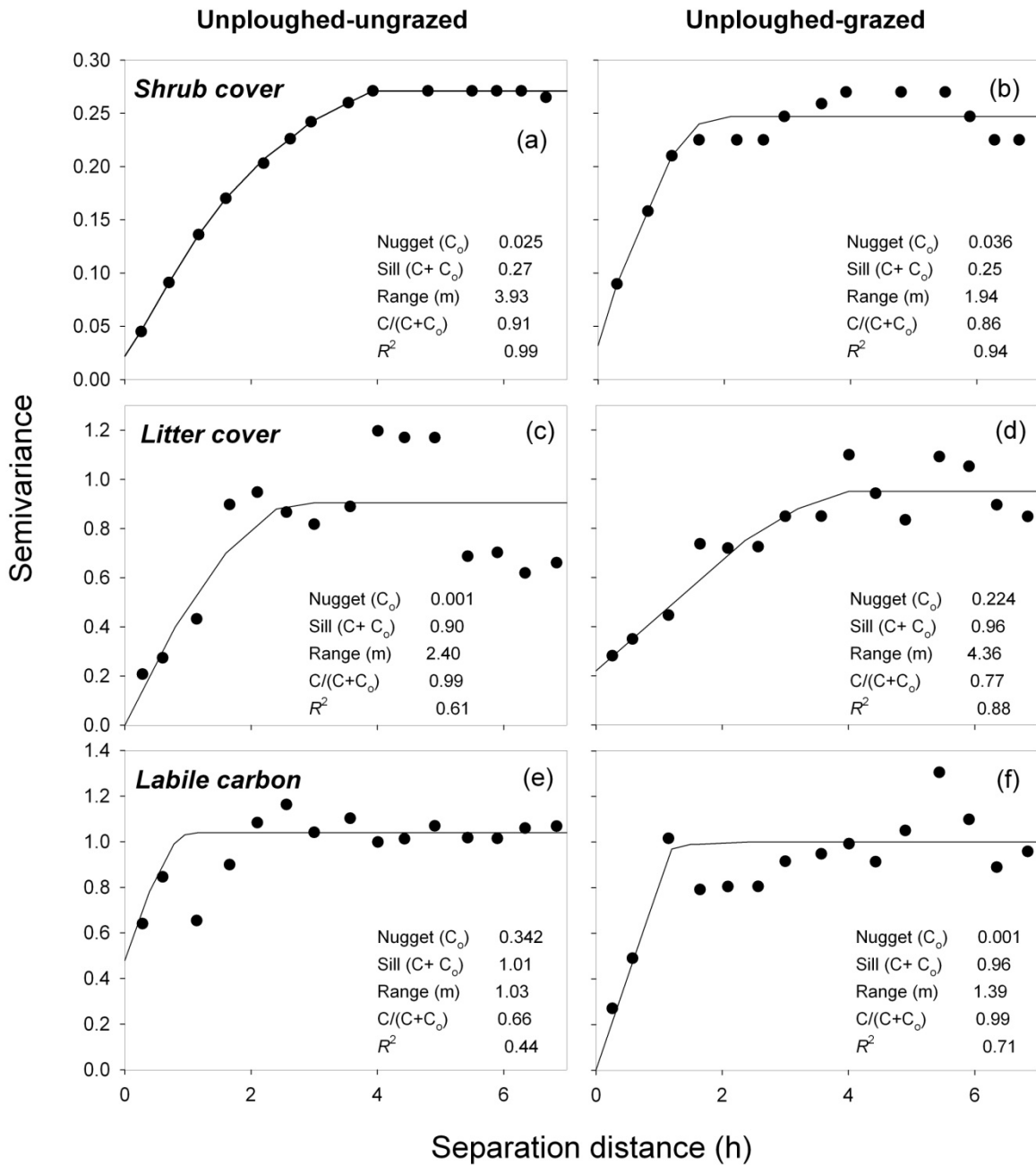
Figure 2. Semivariograms for shrub cover, litter cover and labile C at the unploughed-ungrazed (a, c, e) and unploughed-grazed sites (b, d, f). All semivariograms used spherical models.
