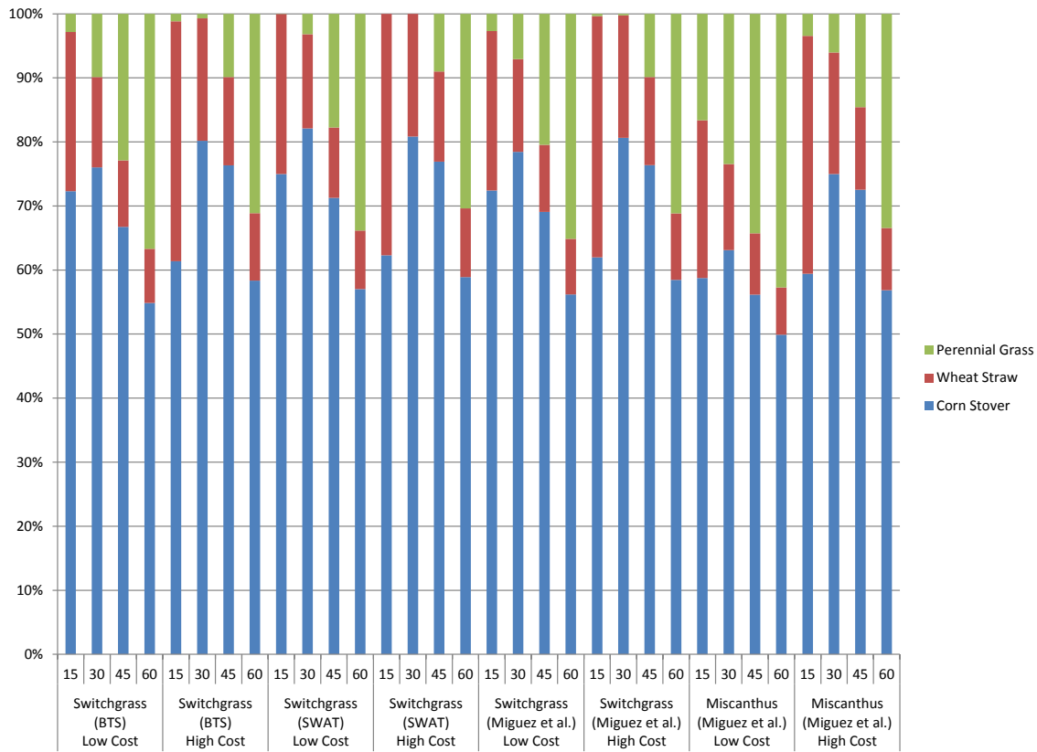
Figure 1: Feedstock Mix
