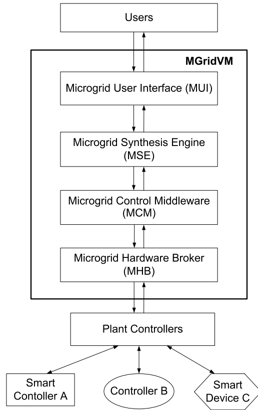
Figure 3.10: MGridVM high-level architecture.
