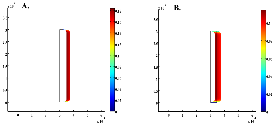
Fig 4.1. Representative strain measurements obtained from 2D finite element, axis symmetric rat mesenteric arteriole model of thickness (A) 25 \mu M (Control) and (B) 45 \mu M (High salt) experiencing 50 mmHg intravascular pressure.
