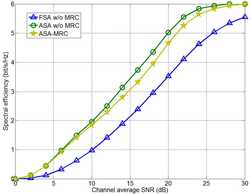
Figure 3.9 Spectral efficiency of fixed sub-carrier allocation scheme (FSA) and proposed adaptive sub-carrier allocation schemes (ASA) in multiuser OFDM systems
