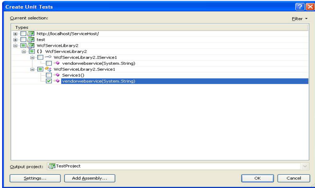
Figure 57: Class Selection
