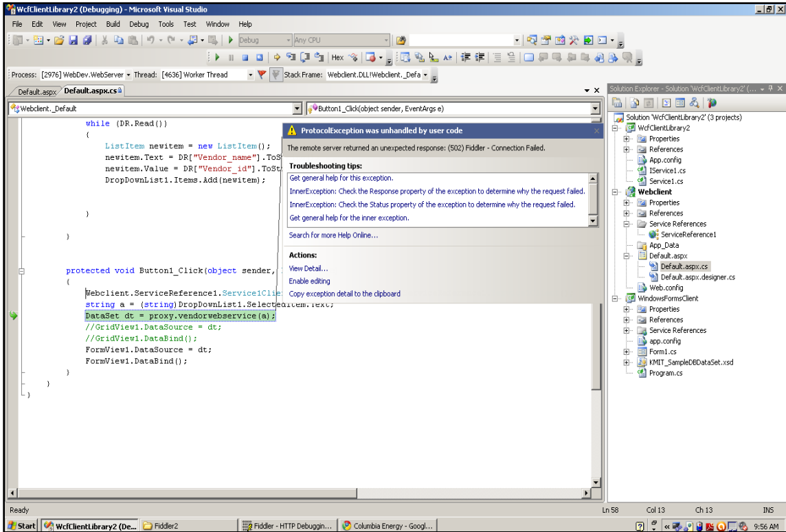
Figure 70: Exception
