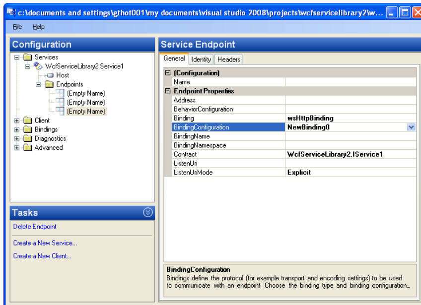
Figure 33: Configuring Endpoint
