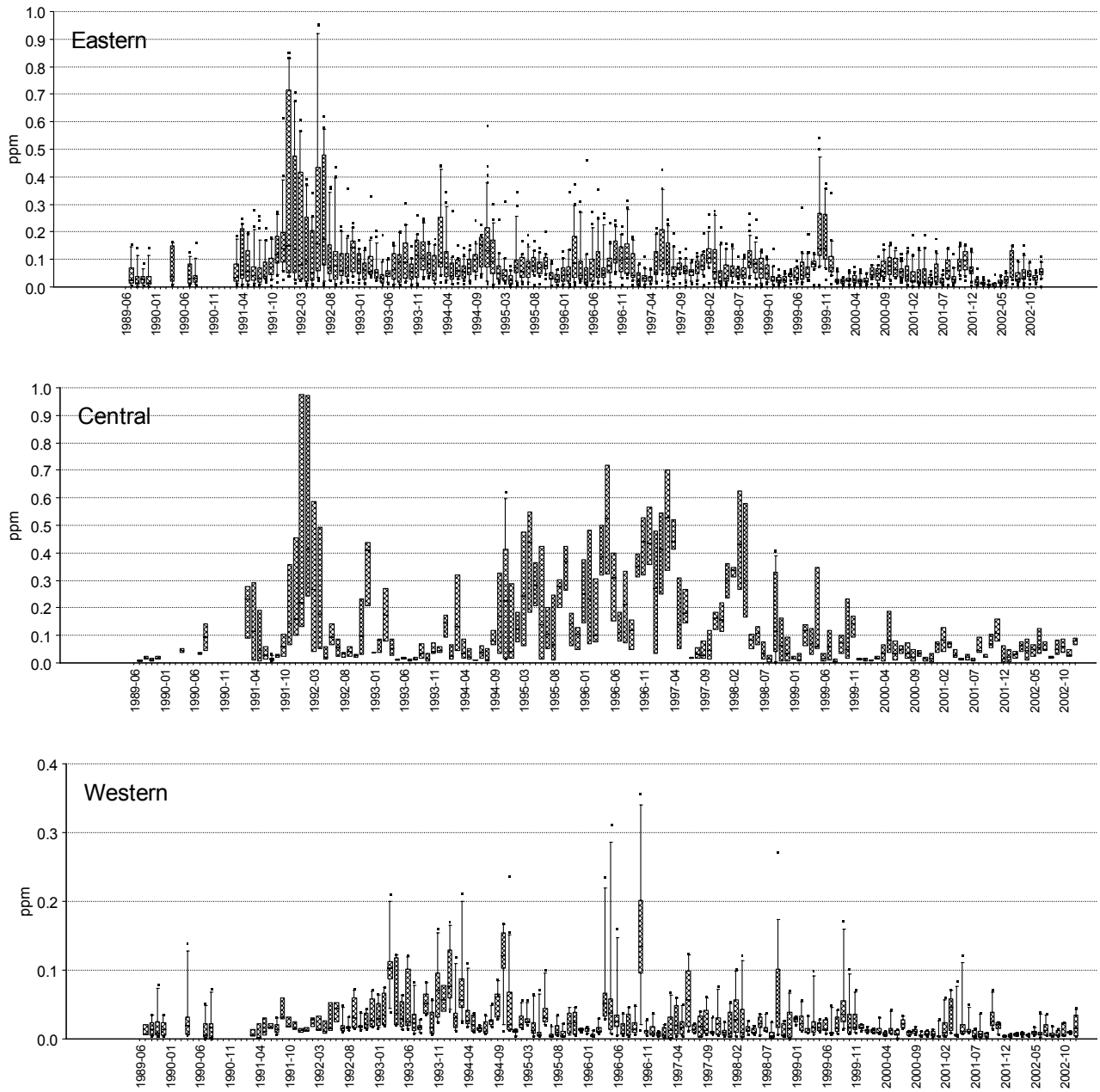
Figure 2.6. Monthly median and range of DIN in the three Florida Bay zones.
