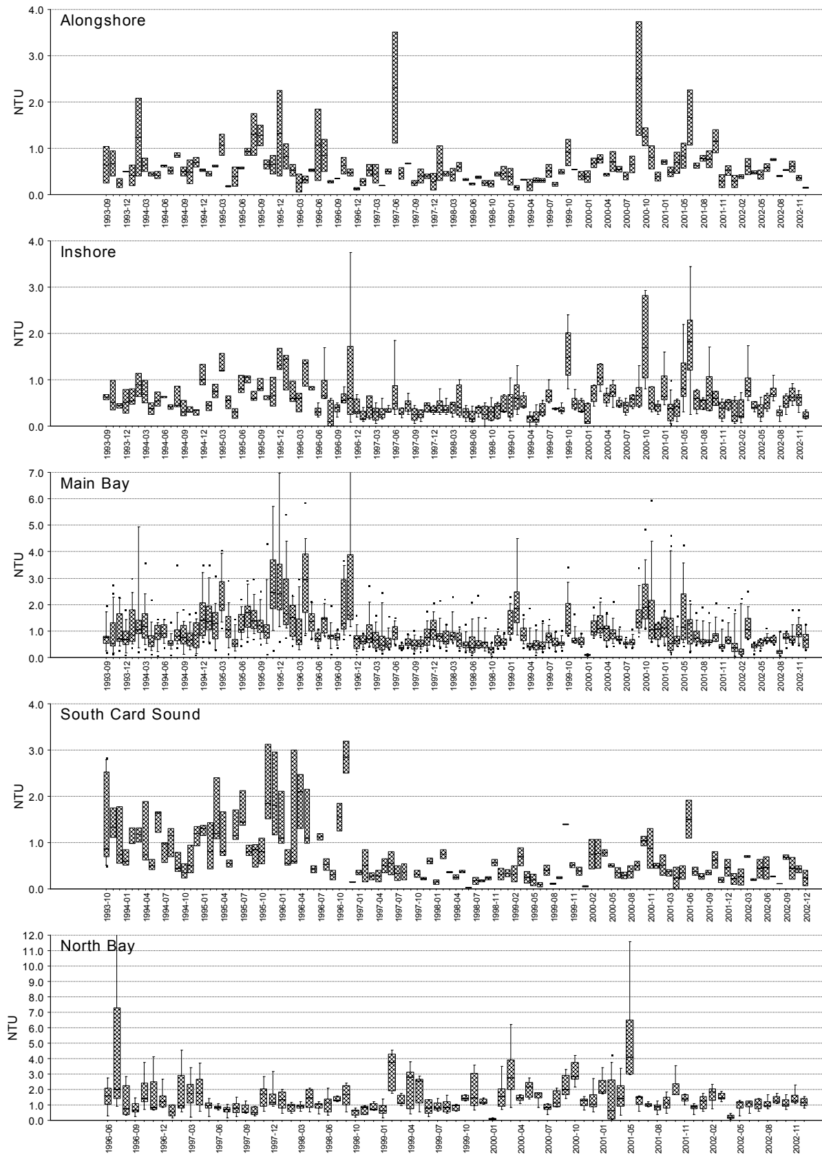
Figure 4.6. Monthly median and range of turbidity in the five Biscayne Bay zones.
