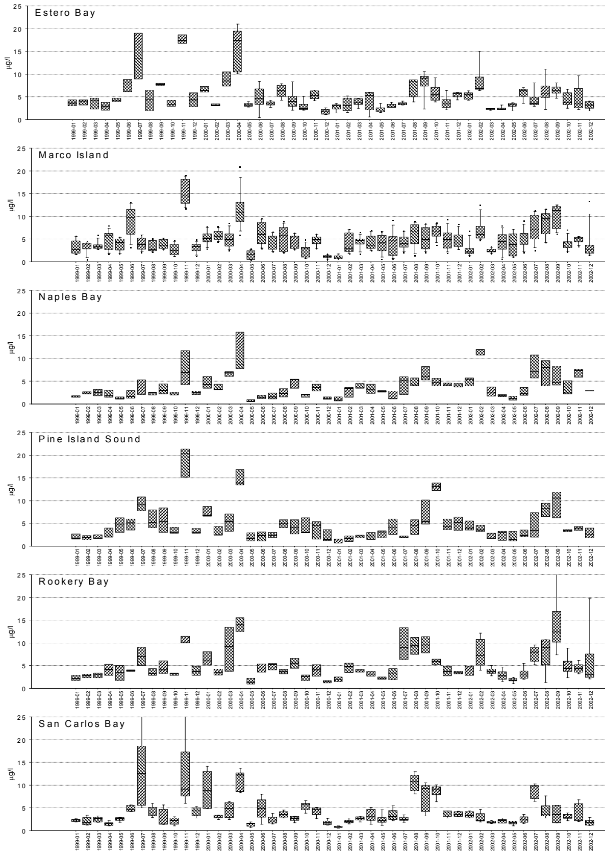
Figure 6.3. Monthly median and range of chlorophyll a in the Cape Romano-PIS area.
