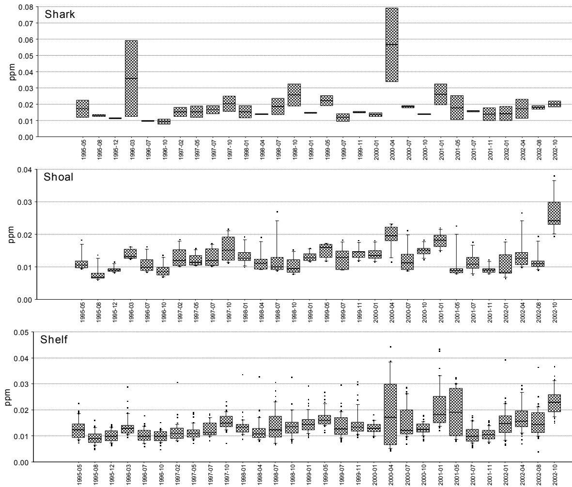
Figure 5.4. Quarterly median and range of total phosphorus in the three SW Shelf zones.
