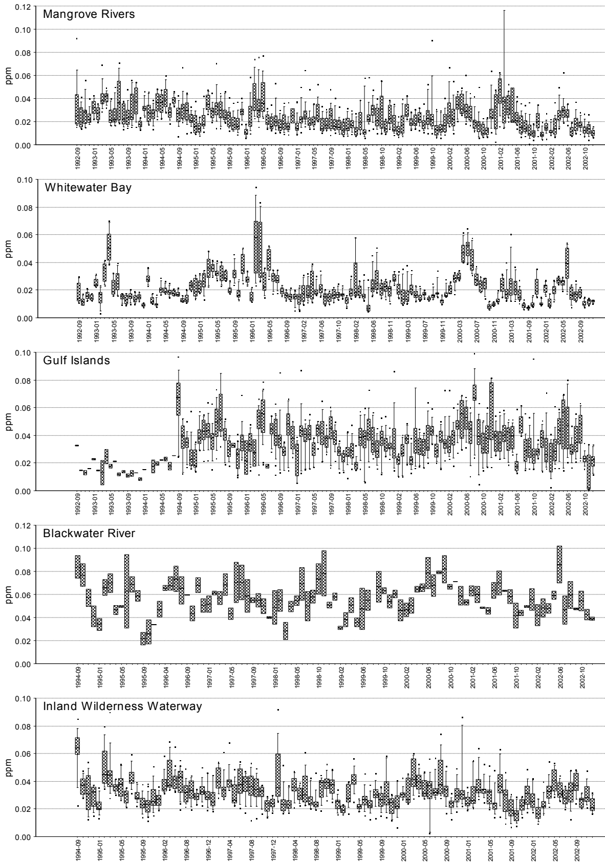
Figure 3.4. Monthly median and range of total phosphorus in the five WWB-TTI zones.
