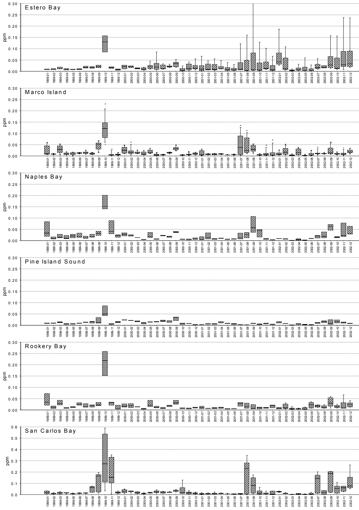
Figure 6.5. Monthly median and range of DIN in the Cape Romano-PIS area.
