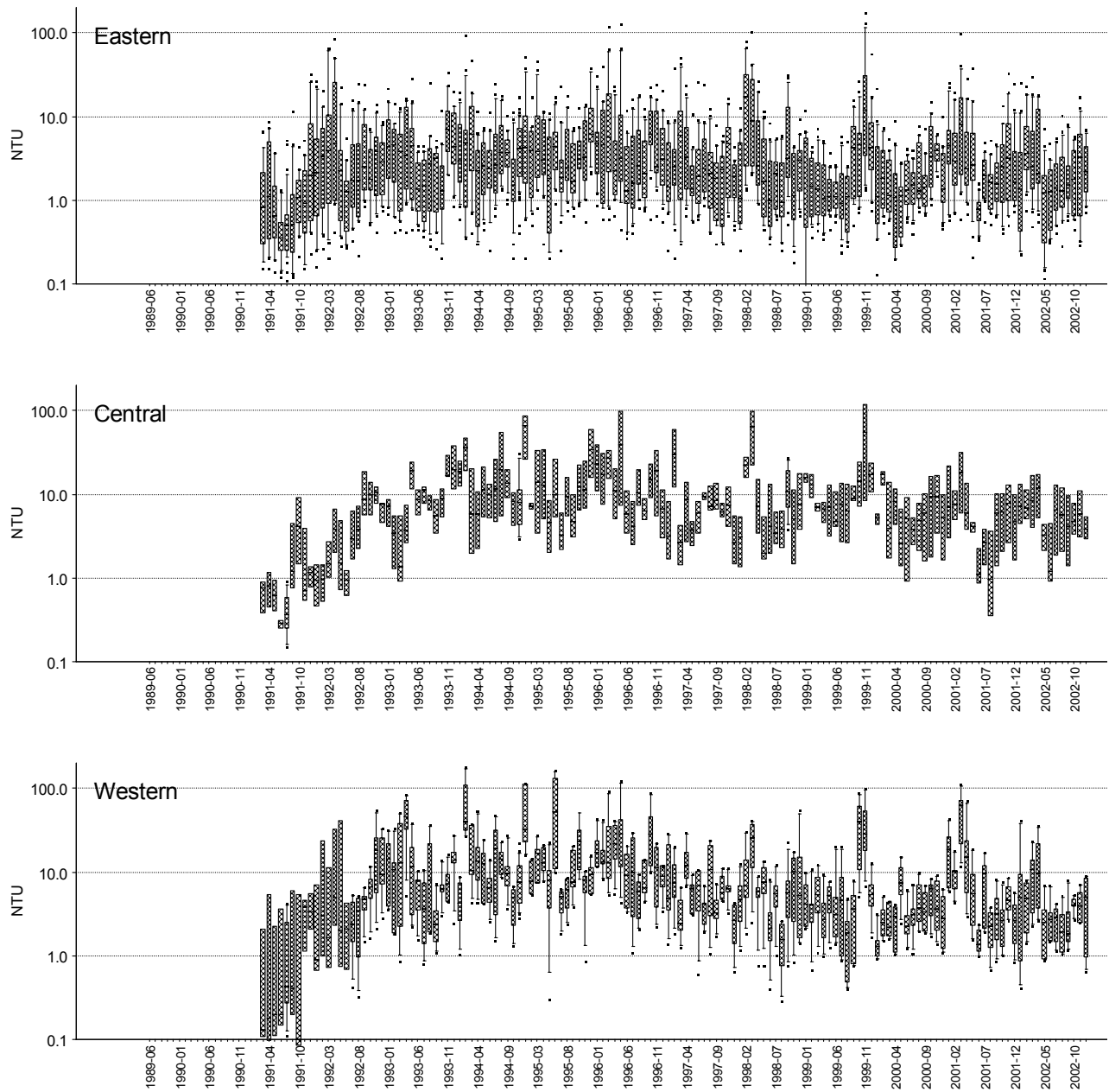
Figure 2.7. Monthly median and range of turbidity in the three Florida Bay zones.
