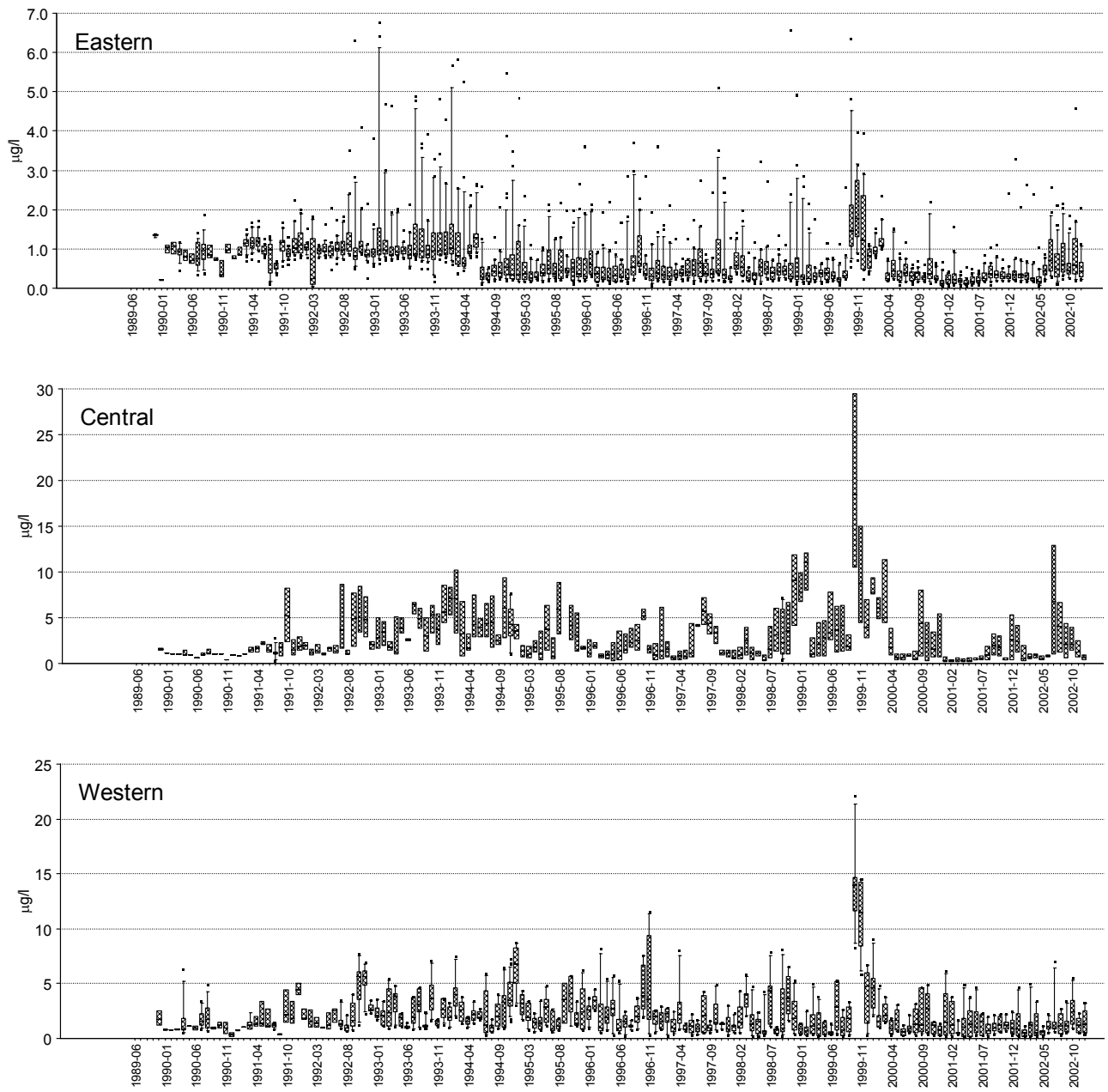
Figure 2.4. Monthly median and range of CHLA in the three Florida Bay zones.
