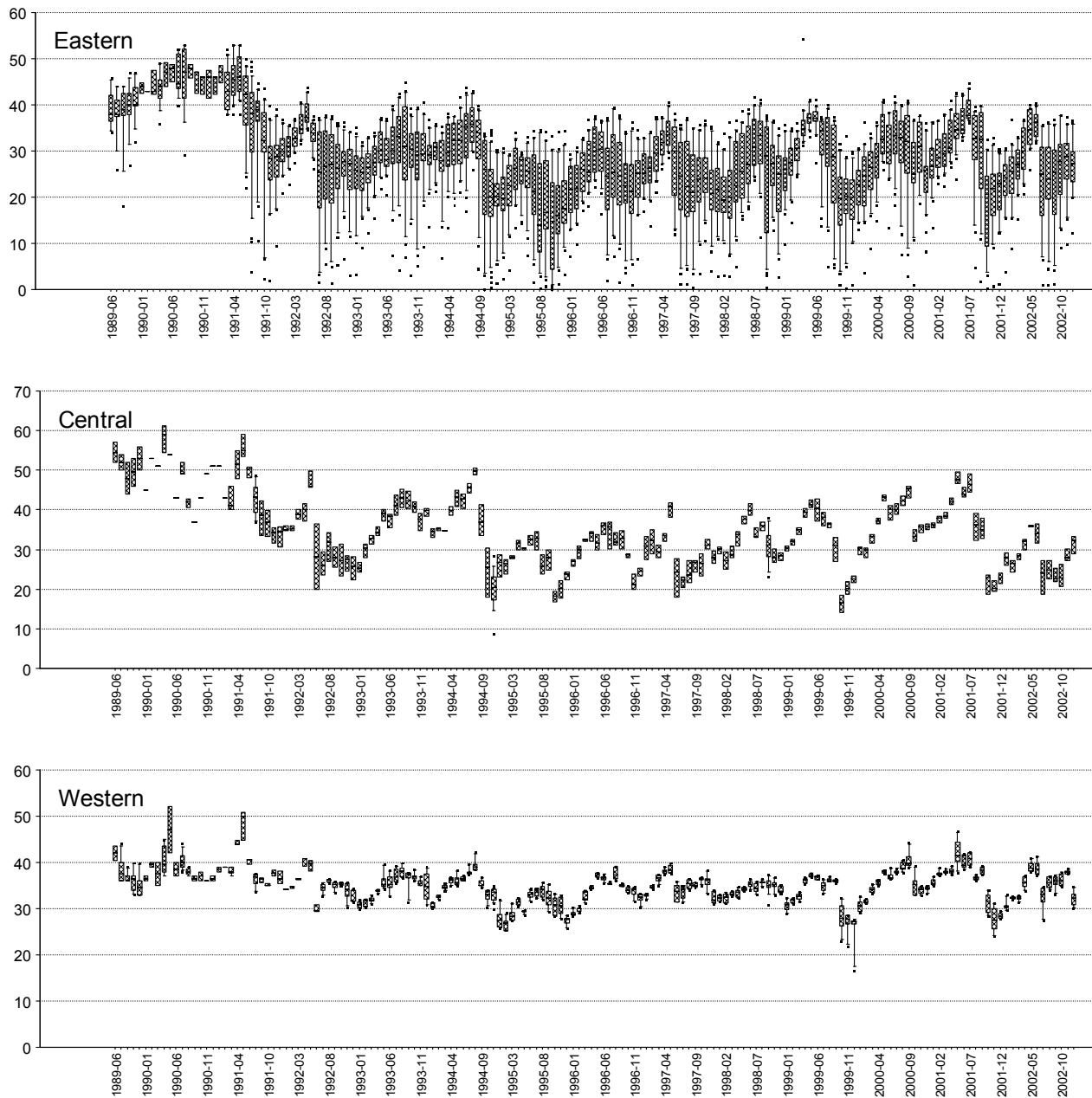
Figure 2.3. Monthly median and range of salinity in the three Florida Bay zones.
