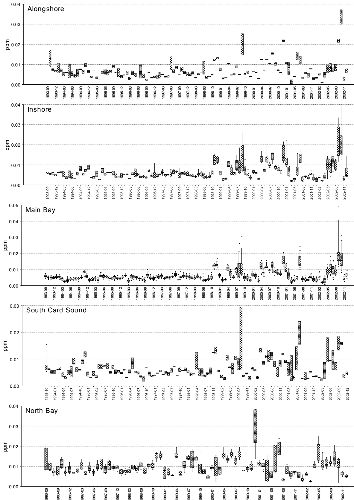
Figure 4.4. Monthly median and range of total phosphorus in the five Biscayne Bay zones.
