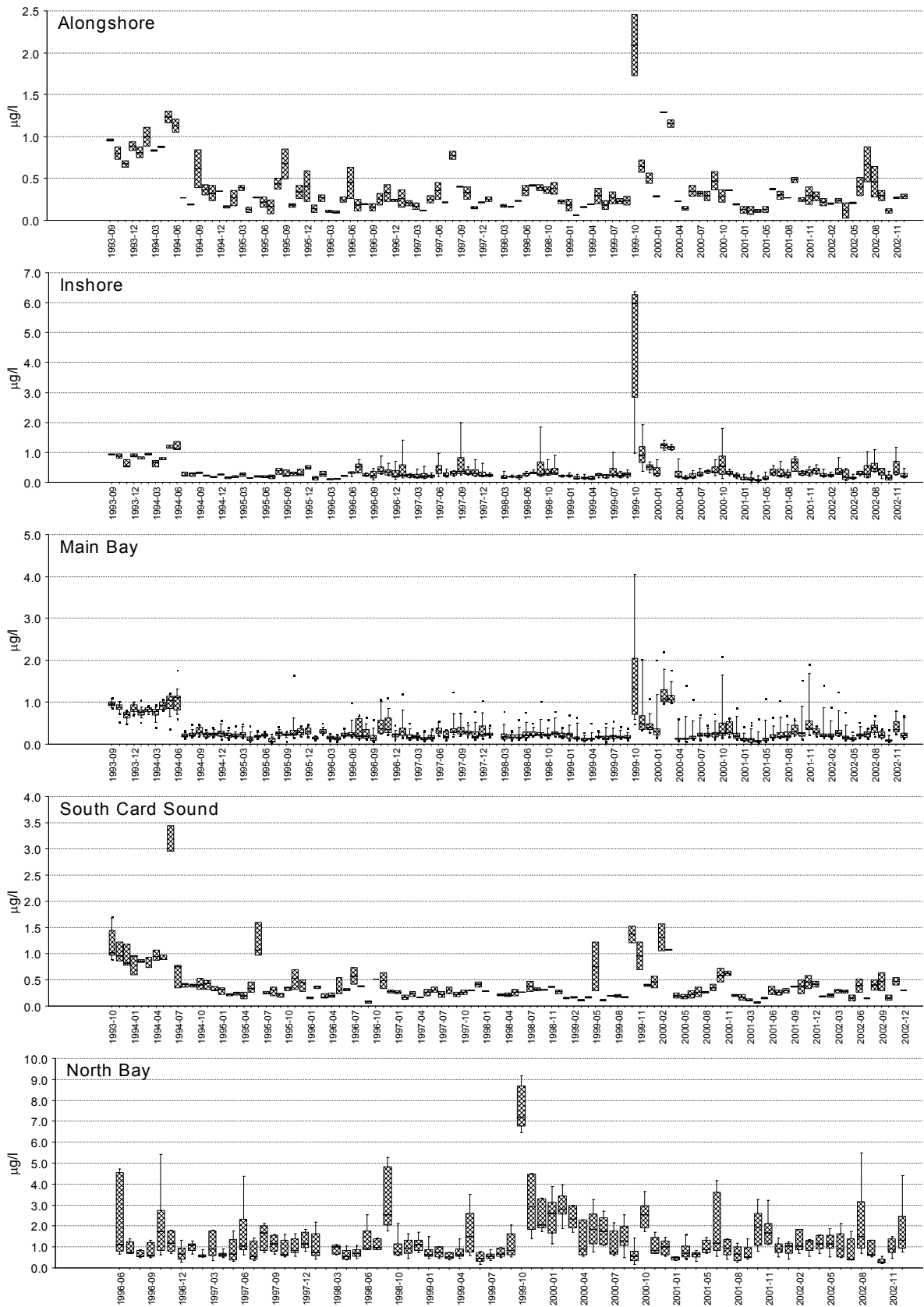
Figure 4.3. Monthly median and range of chlorophyll a in the five Biscayne Bay zones.
