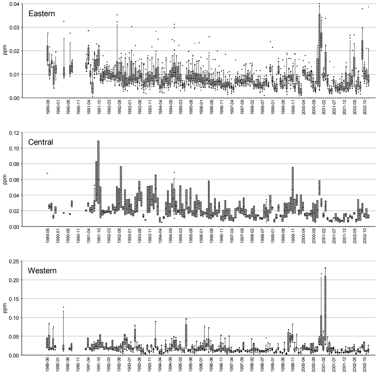
Figure 2.5. Monthly median and range of TP in the three Florida Bay zones.
