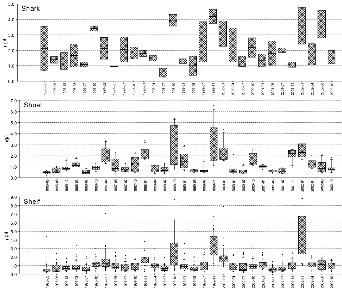
Figure 5.3. Quarterly median and range of chlorophyll a in the three SW Shelf zones.
