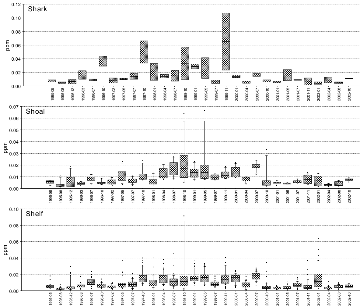
Figure 5.5. Quarterly median and range of dissolved inorganic N in the three SW Shelf zones.
