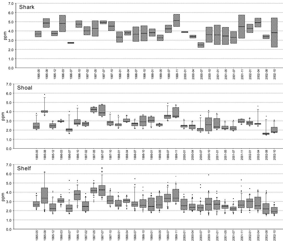
Figure 5.6. Quarterly median and range of total organic carbon in the three SW Shelf zones.
